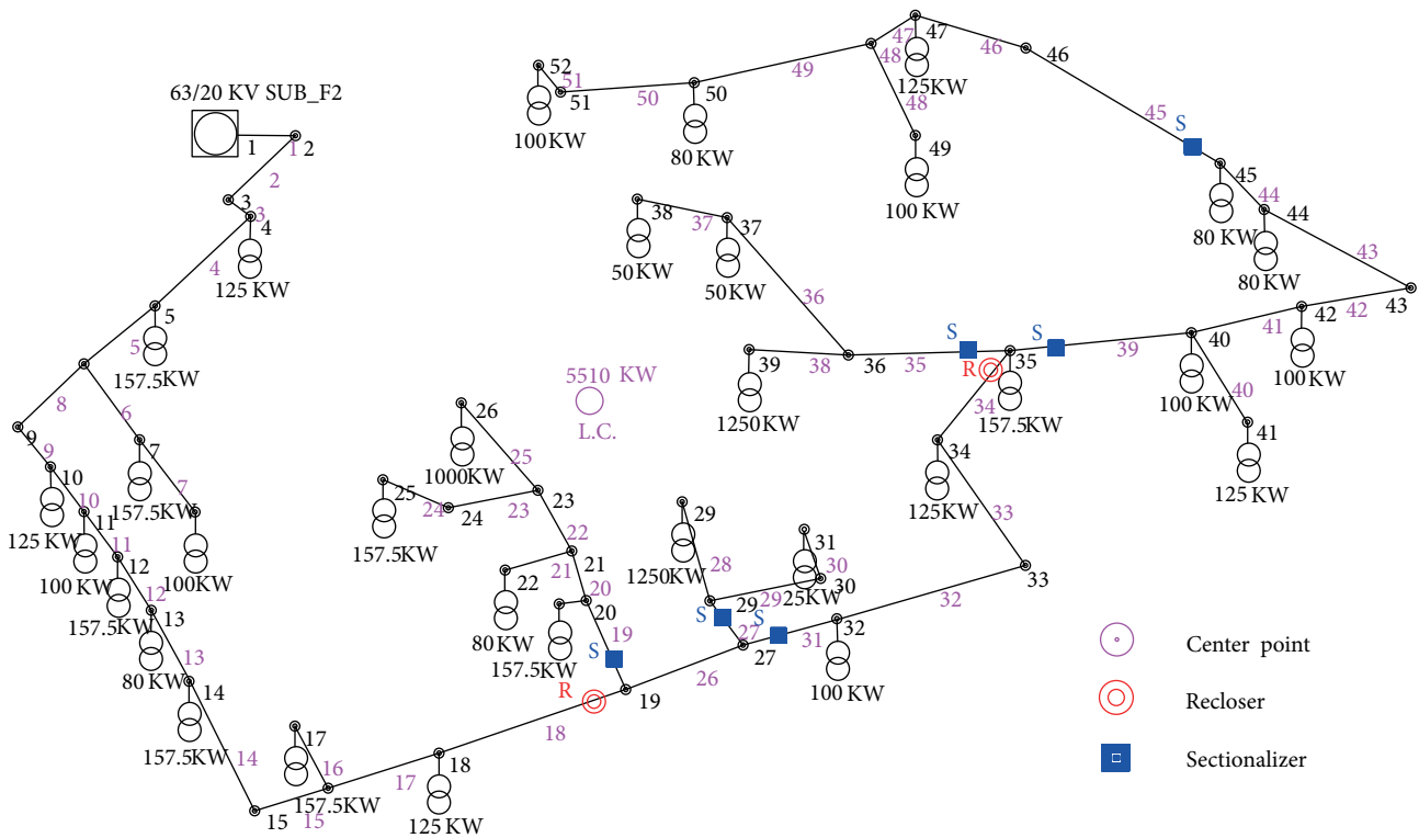
Figure 7. Optimal locations of AR/S in feeder F2 with RFa.
