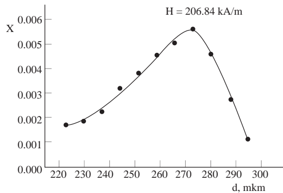
Figure 4. The relationship between the magnetic susceptibility of PMMS-IVb and diameter.
