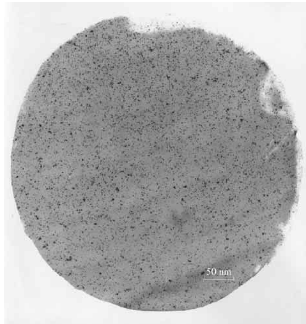
Figure 2a. Electron microphotography of PMMS-IVb section at magnification 50000.
