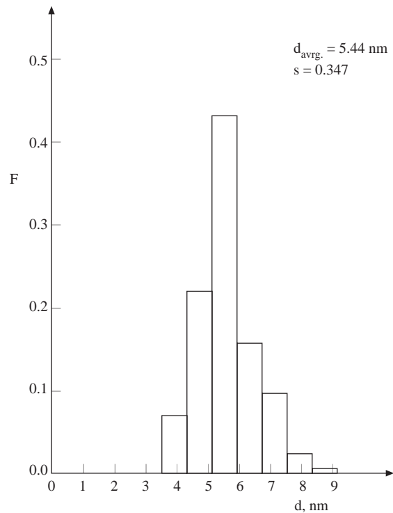
Figure 2b. Histogram of the distribution of magnetite nanoparticles by size.
