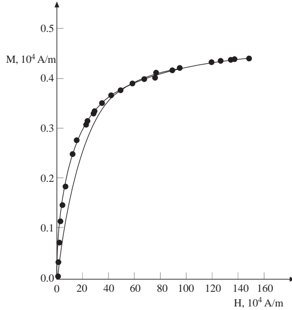
Figure 3. Magnetization curves of PMMS-IVb, obtained at concentration of magnetite nanoparticles \varphi_m = 0.000984 by vibration sample magnetometry (line+symbols) and calculated by Langevan equation (solid line).
