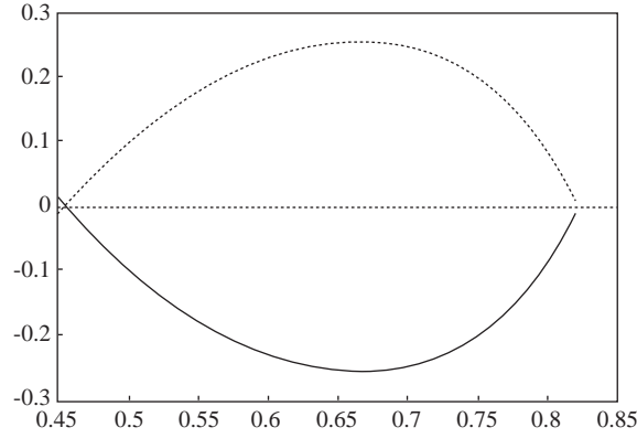
Figure 5. The dependence of \mathcal{N} on \hat{s} for B \rightarrow K\tau^+\tau^- decay which corresponds to the cases : C_{LRLR} = -C_{10} (top curve), C_{LRLR} = C_{10} (bottom curve).
