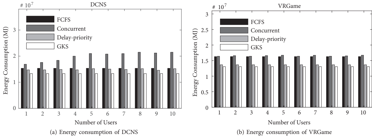
Figure 10. Comparison of energy consumption by FCFS, concurrent, delay-priority, and GKS based on the number of users.
