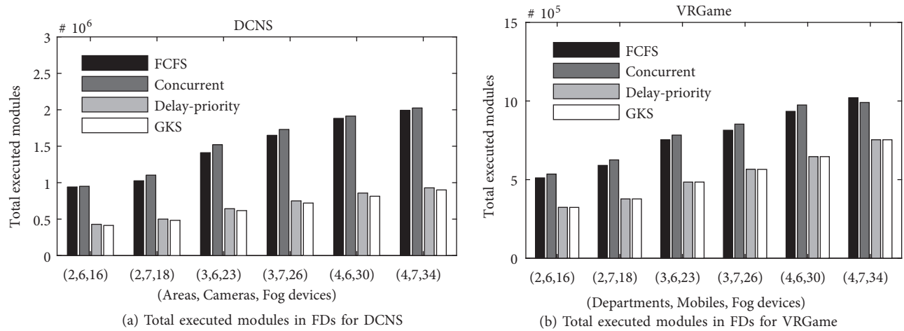
Figure 4. Total executed modules in FDs.
