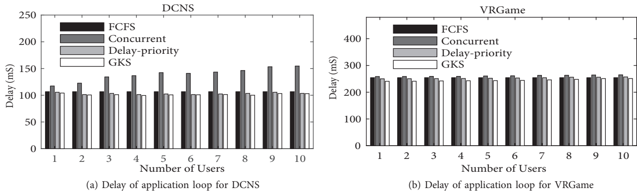
Figure 12. Comparison of delay of application loop by FCFS, concurrent, delay-priority, and GKS based on the number of users
