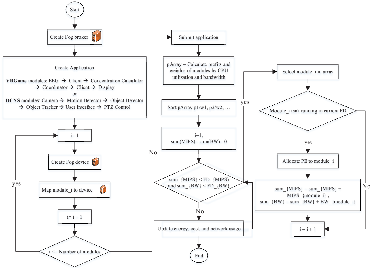
Figure 3. The flowchart of GKS.
