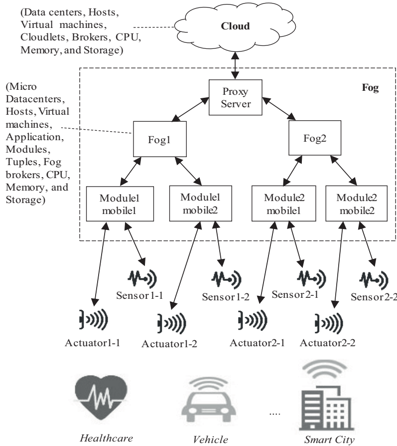
Figure 1. Fog computing architecture.
