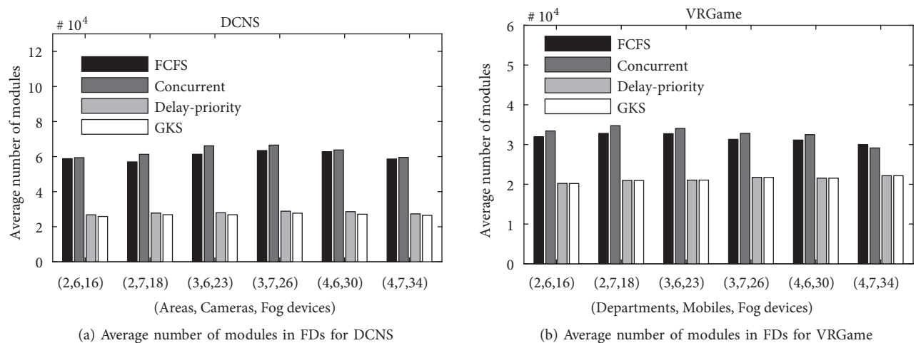
Figure 5. Average number of modules in FDs.
