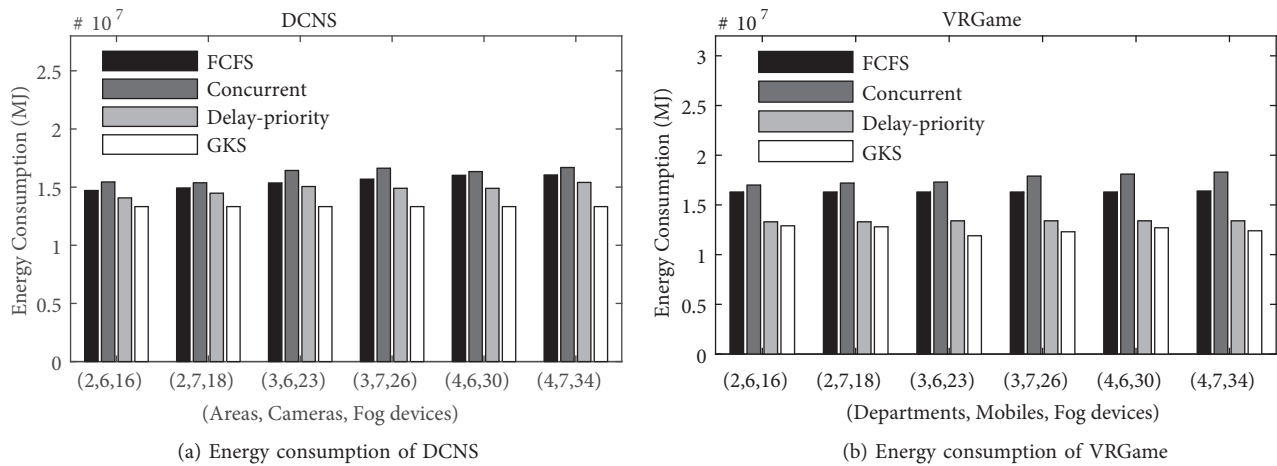
Figure 8. Energy consumption of FCFS, concurrent, delay-priority, and GKS
