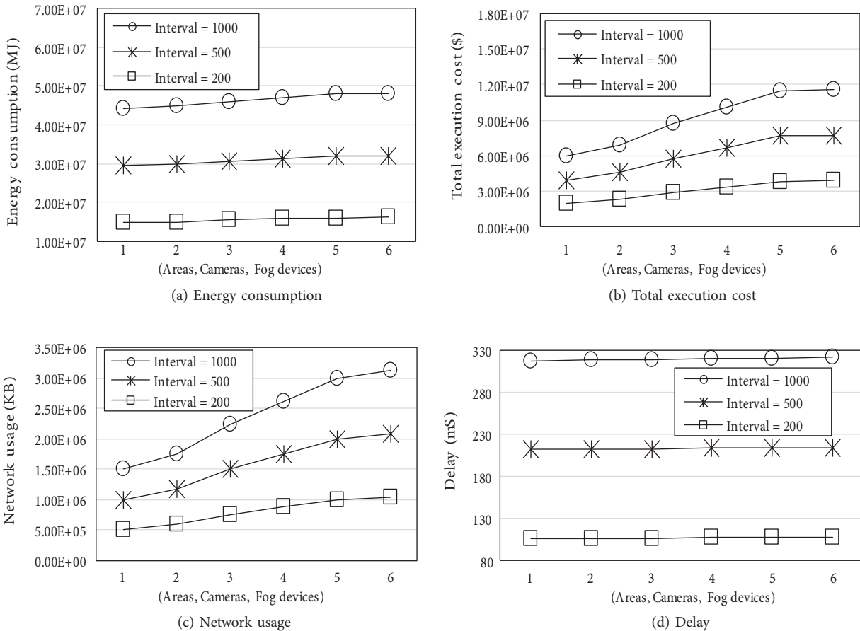
Figure 6. Analysis GKS algorithm based on resource management intervals of DCNS.
