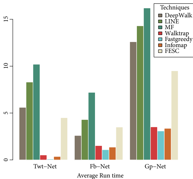
Figure 4. Results of average running time of FESC compared with baseline frameworks. Running time of network embedding techniques is high due to nonsharing of parameters. FESC and community discovery techniques had a time complexity of \sim O(V + E) , resulting in lower running time.
