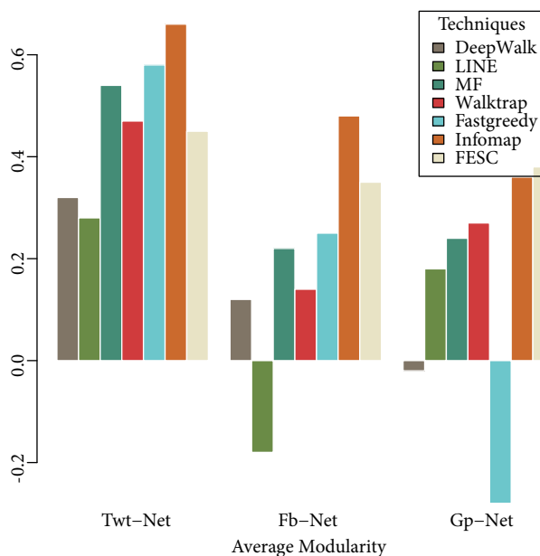
Figure 2. Results of average modularity metric in comparison of FESC with baseline frameworks. Modularity optimizing algorithms such as Walktrap and Fastgreedy identified community structure with high modularity. Infomap technique based on minimizing the expected description length of a random walkers trajectory outperformed other techniques. Network embedding techniques with embedding dimensions set to 5 resulted in low modularity partitions. Performance of FESC is comparative to community discovery techniques.
