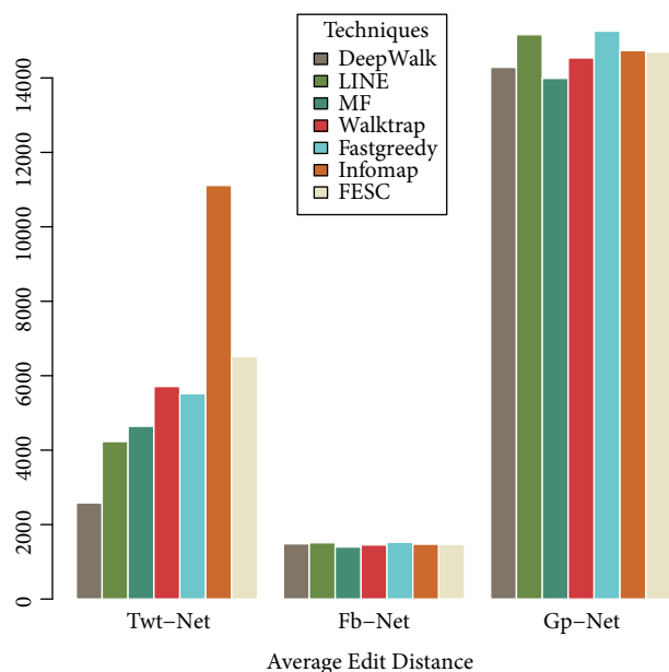
Figure 3. Results of average edit distance metric in comparison of FESC with baseline frameworks. Modules discovered by community detection frameworks do not correspond to social circle communities and hence the value of the edit distance metric was high for modularity maximizing techniques such as Walktrap and Fastgreedy. Network embedding techniques fared relatively better than community discovery techniques. FESC performed better than modularity maximization and random walk-based techniques of community discovery.
