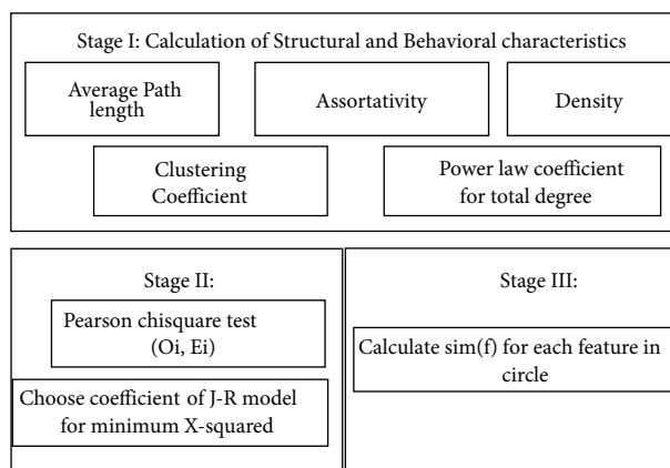
Figure 1. Block diagram of FESC algorithm shows the components of the three stages and individual components of each stage. The statistical features of the ego-nets are extracted from the social networks in Stage I. Stage II uses the J-R model to understand the characteristics of the degree distribution. The third stage provides a similarity value for each feature of the ego using the attribute information of the alters.
