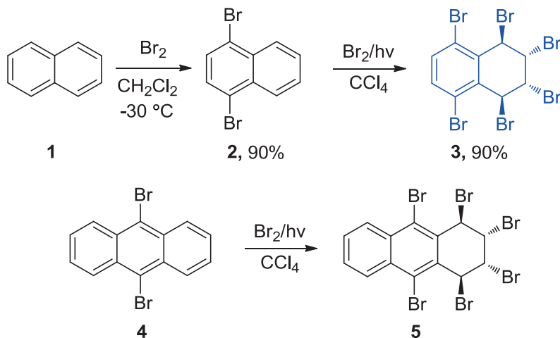
Scheme 1. Polar and photobromination of naphthalene ( 1 ) and 9,10-dibromoanthracene ( 4 ).
