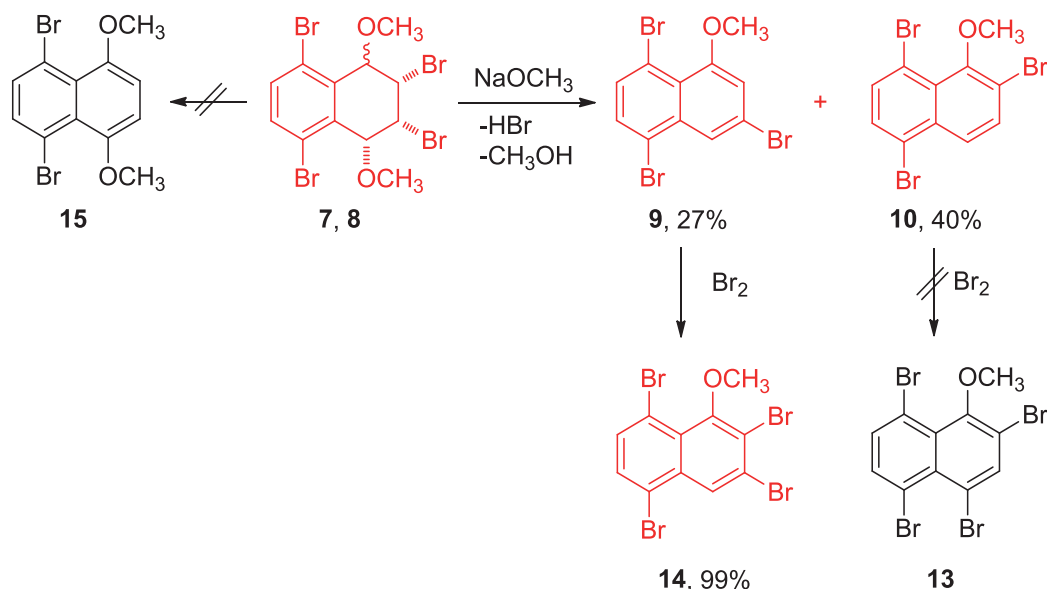
Scheme 6. Aromatization of dimethoxides 7 and 8 , followed by electrophilic bromination.
