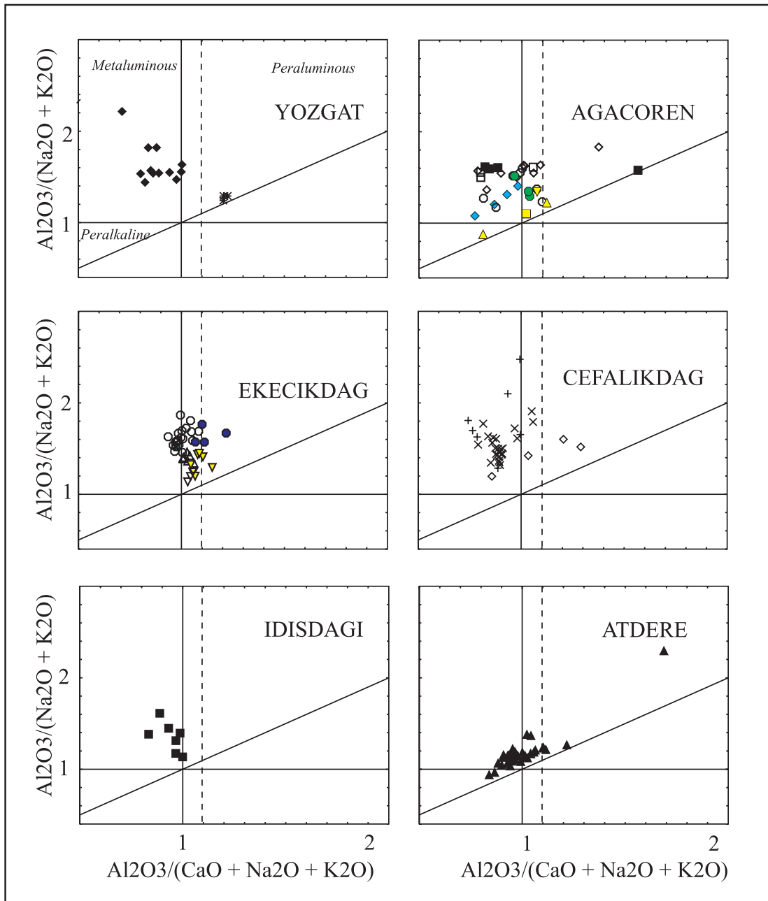
Figure 4. Shand Index diagram after Maniar and Piccoli (1989). Symbols as in Fig. 2.
