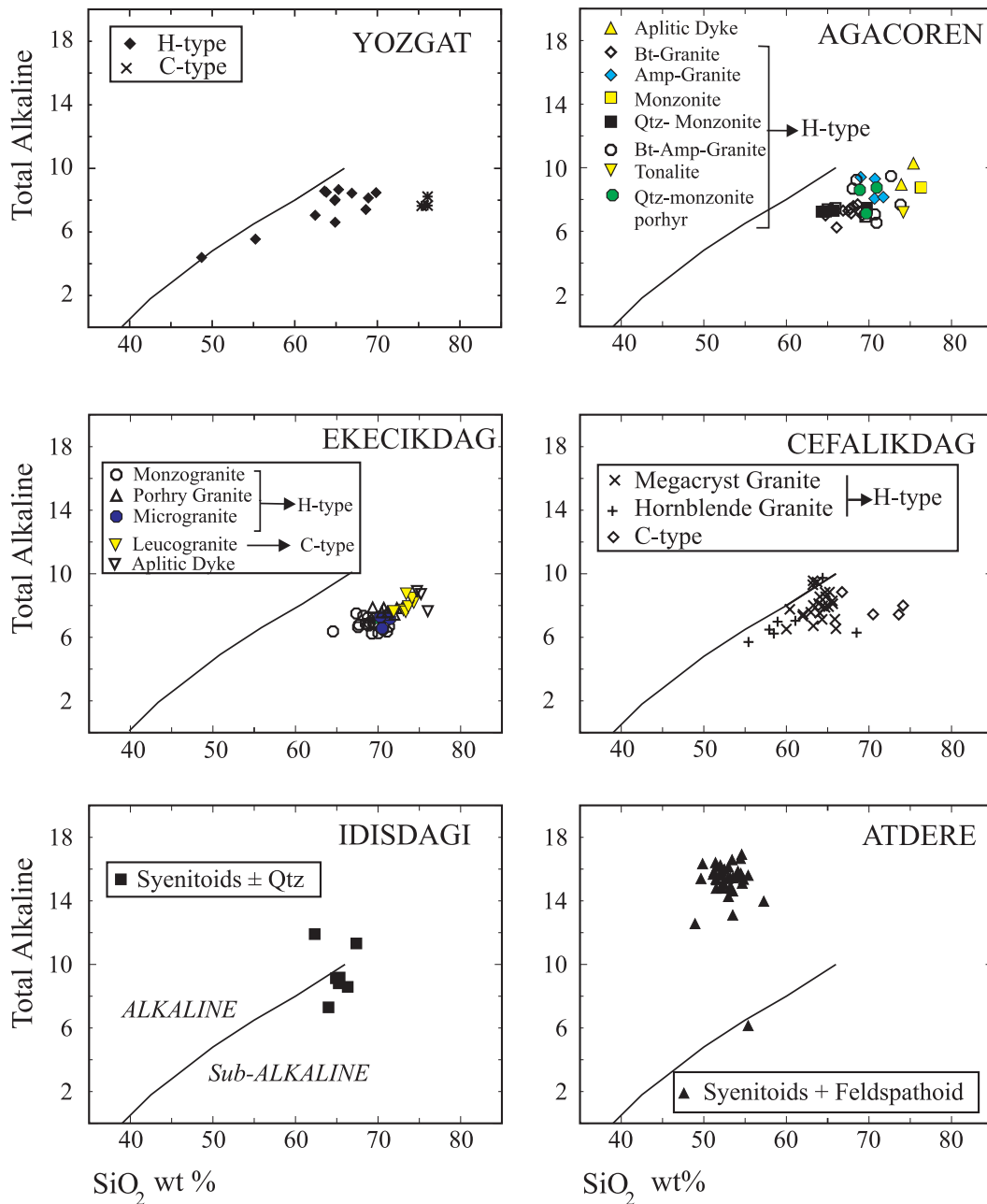
Figure 2. Plots of the total alkali versus SiO 2 diagram where alkaline and subalkaline fields are from Irvine and Baragar (1971).
