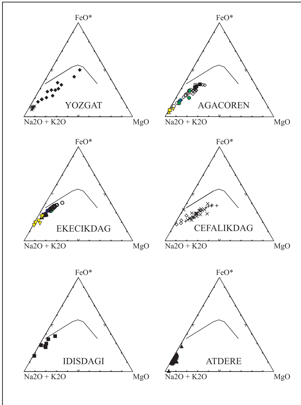
Figure 3. Plots of AFM diagram where tholeiitic and calc-alkaline fields are from Irvine and Baragar (1971). Symbols as in Fig. 2.
