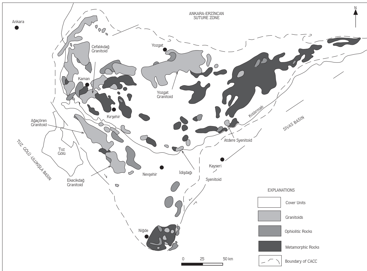
Figure 1. Location map and simplified geological setting of the Central Anatolian Crystalline Complex.
