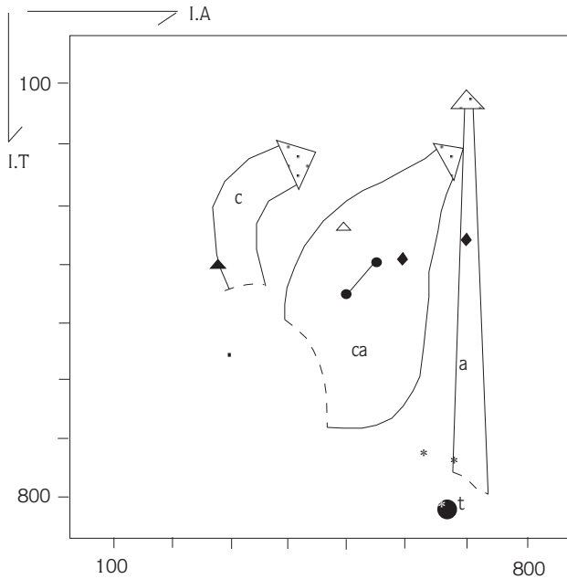
Figure 7. Distribution of the mean points compared to the main typological trends of zircon populations in granitic rocks. c: crystal-derived granites. ca: calc-alkaline series. a: alkaline series. t: plagiogranites or trondhjemites. Black triangle: Piyi migmatites, open triangle: associated aplite. Dots: Fanos granite. Rhombs: matrix of magmatic breccias. Stars: trondhjemites. I.A: index related to appacity, I.T: index related to temperature of crystallization.
