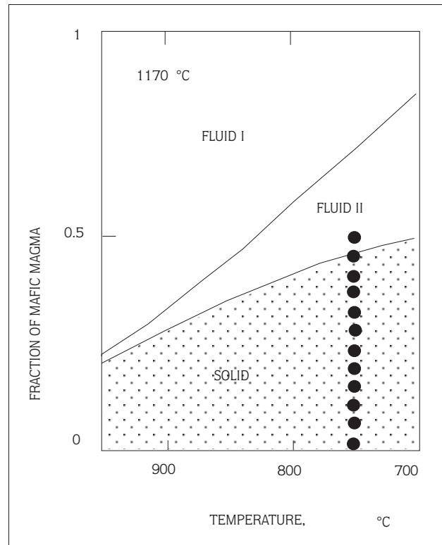
Figure 12. Location of the hybrid rocks of Porto in the silicic magma-mixing diagram of Sparks and Marshall (1986).
