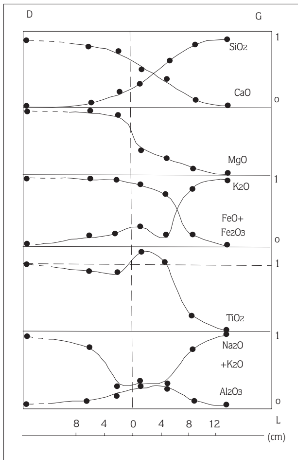
Figure 5. Normalized oxide variation diagrams in the quartz diorite-granite association (Porto complex). Normalized is made between quartz diorite D and granite G compositions (wt. %). Data are plotted against the distance L from the interface between basic and acid rocks.
