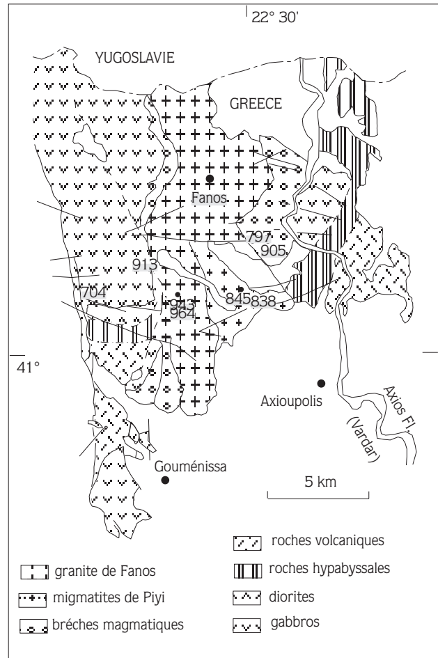
Figure 6. Simplified geological map of the Guevgueli complex.
