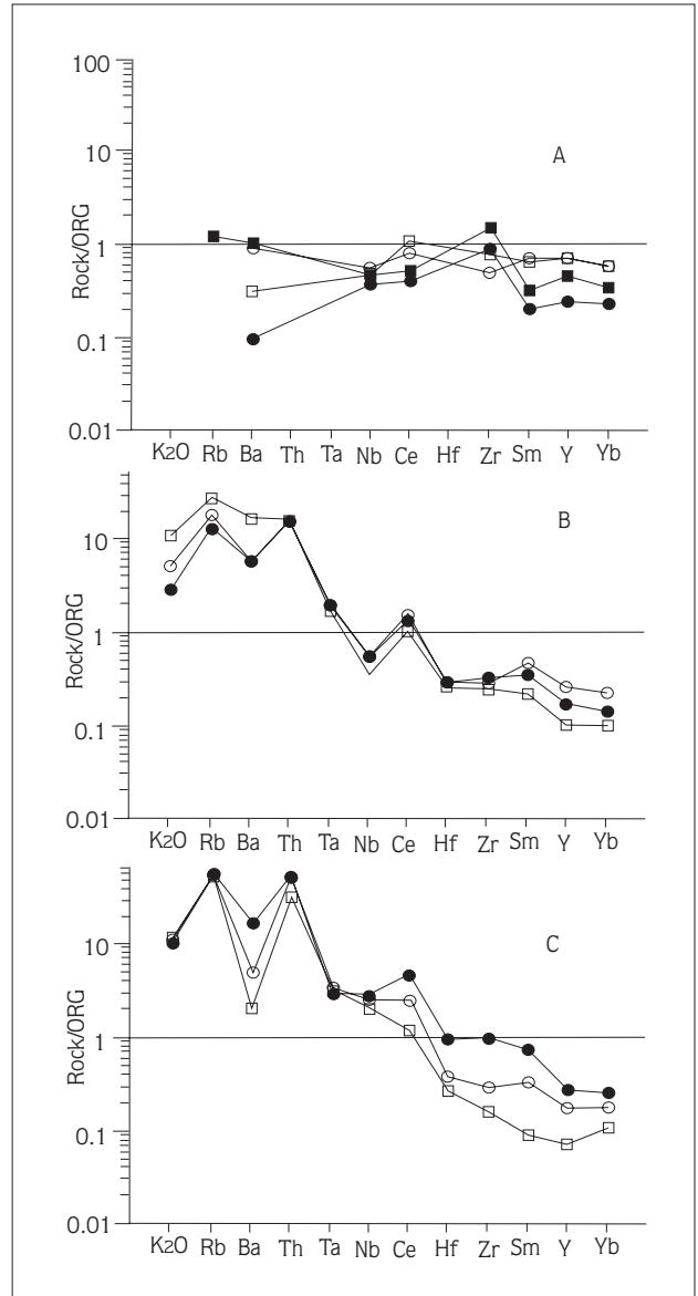
Figure 8. Rock / ORG Spider diagrams for the acidic rocks of the Guevgueli complex (ORG normalization values have been taken after Pearce et al., 1984). A: matrix of magmatic breccias and plagiogranites. B: migmatites of piyi and aplite. C: granite of Fanos.
