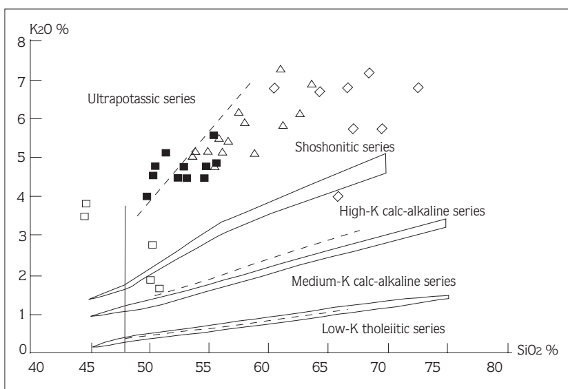
Figure 10. K_2O versus SiO_2 diagram. Open square: Diorites; Black squares: monzogabbro-diorites; Triangles: monzonites; Rhombss: quartz-monzonites and syenites.
