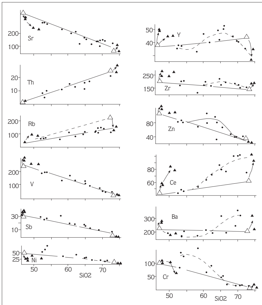
Figure 4. Trace elements versus silica in the Porto association. Dots: monzogranites, granodiorites and quartz diorites. Open triangles: granite and gabbro. solid triangles: granite and gabbro into contact.
