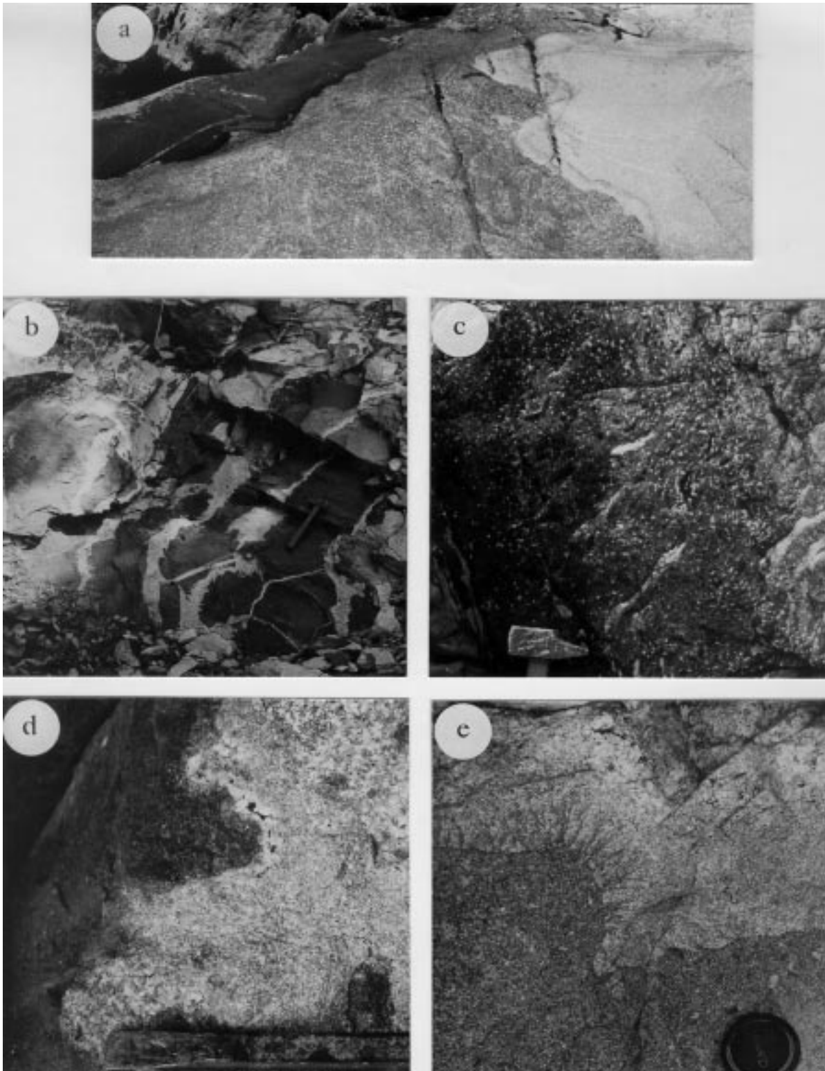
Figure 2. a: association of gabbro, magmatic breccias and granite. b: net-veined complex between gabbro and granite. c: formation of magmatic breccias. d: pegmatitic pocket along the contact between gabbro and granite. e: tree-like structures between quartz-diorite and granite, note the 15 cm thick intermediate rock-type.
