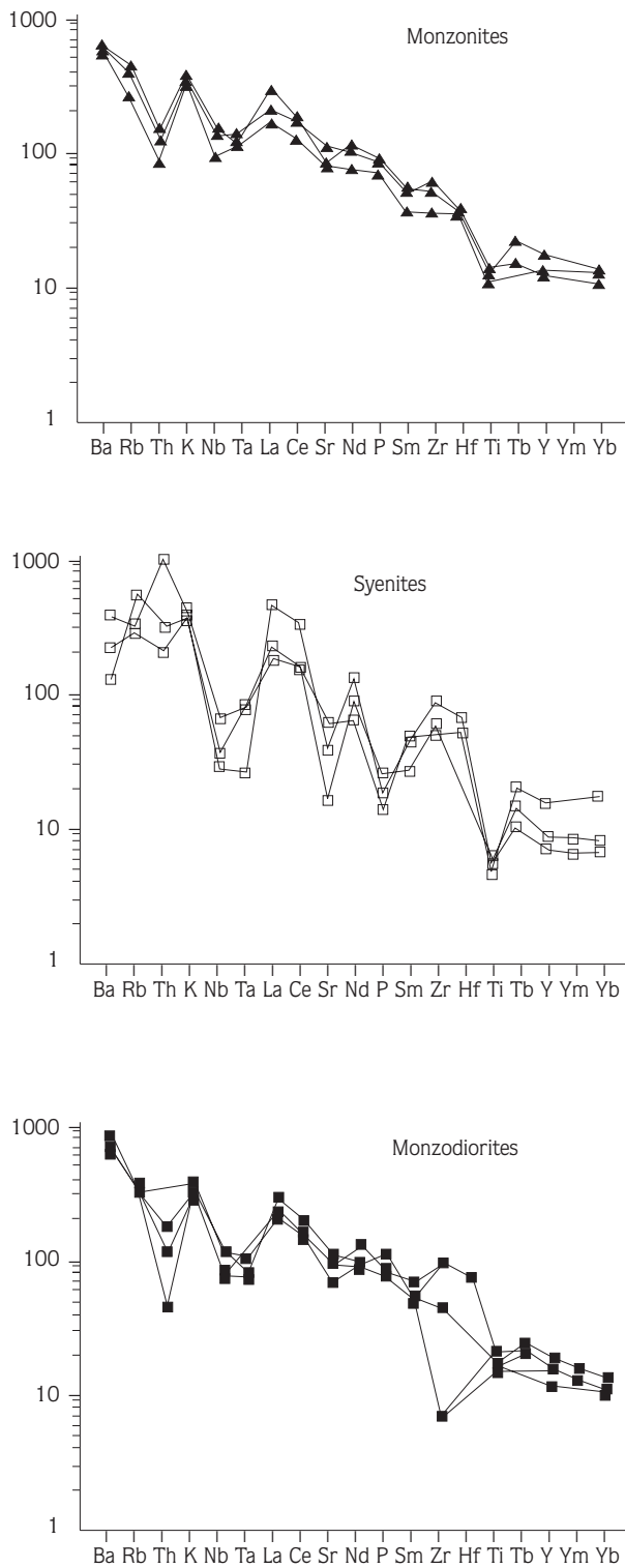
Figure 11. Chondrite-normalized spidergrams (Thomson, 1982) for the Piracaia complex.
