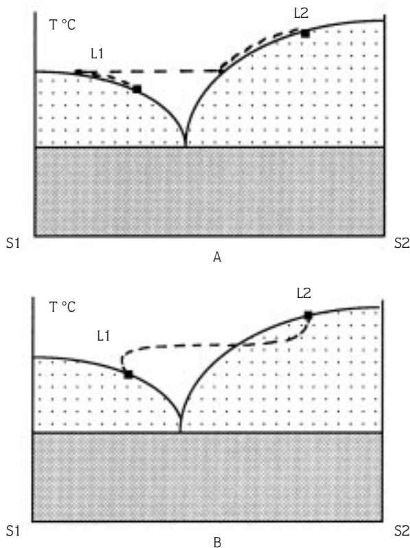
Figure 13. Schematic binary diagrams showing the mixing patterns between the two melts. A: in equilibrium conditions, after remelting its phenocrysts, L1 mixes with L2 for every ratio L1/L2. B: L1 leaves its liquidus before the phenocrysts are totally remelted, L2 is undercooled, the mixing process takes place in disequilibrium conditions, the hybrid melts are undercooled for high ratio of mafic component.
