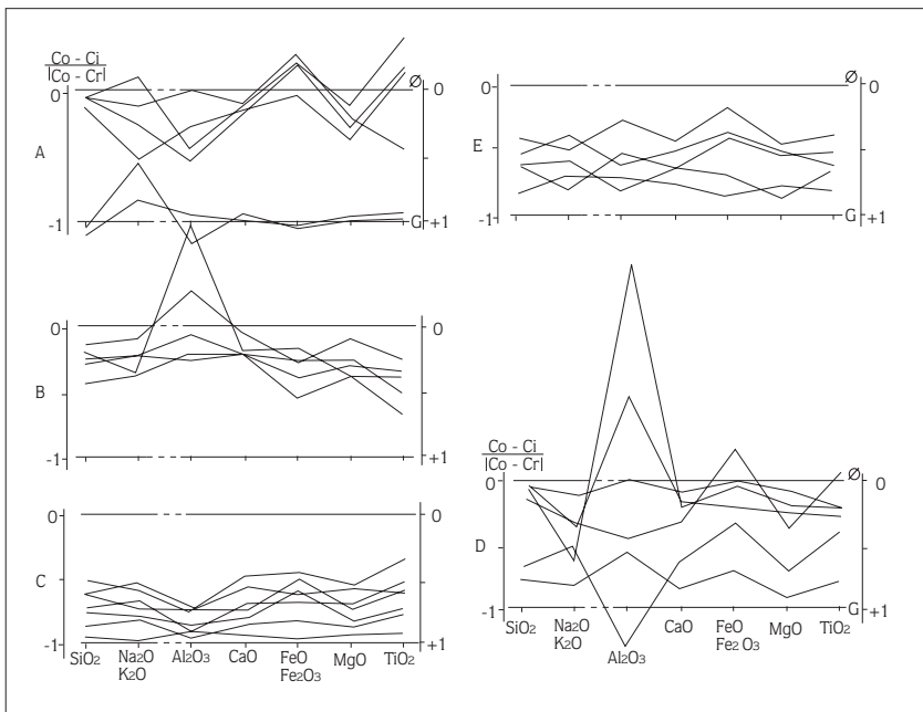
Figure 3. Normalized diagrams for Porto association. A: gabbro and granite into contact. B: quartz-diorite. C: monzogranites and granodiorites. D: enclaves within magmatic breccias. E: matrix of magmatic breccias.
