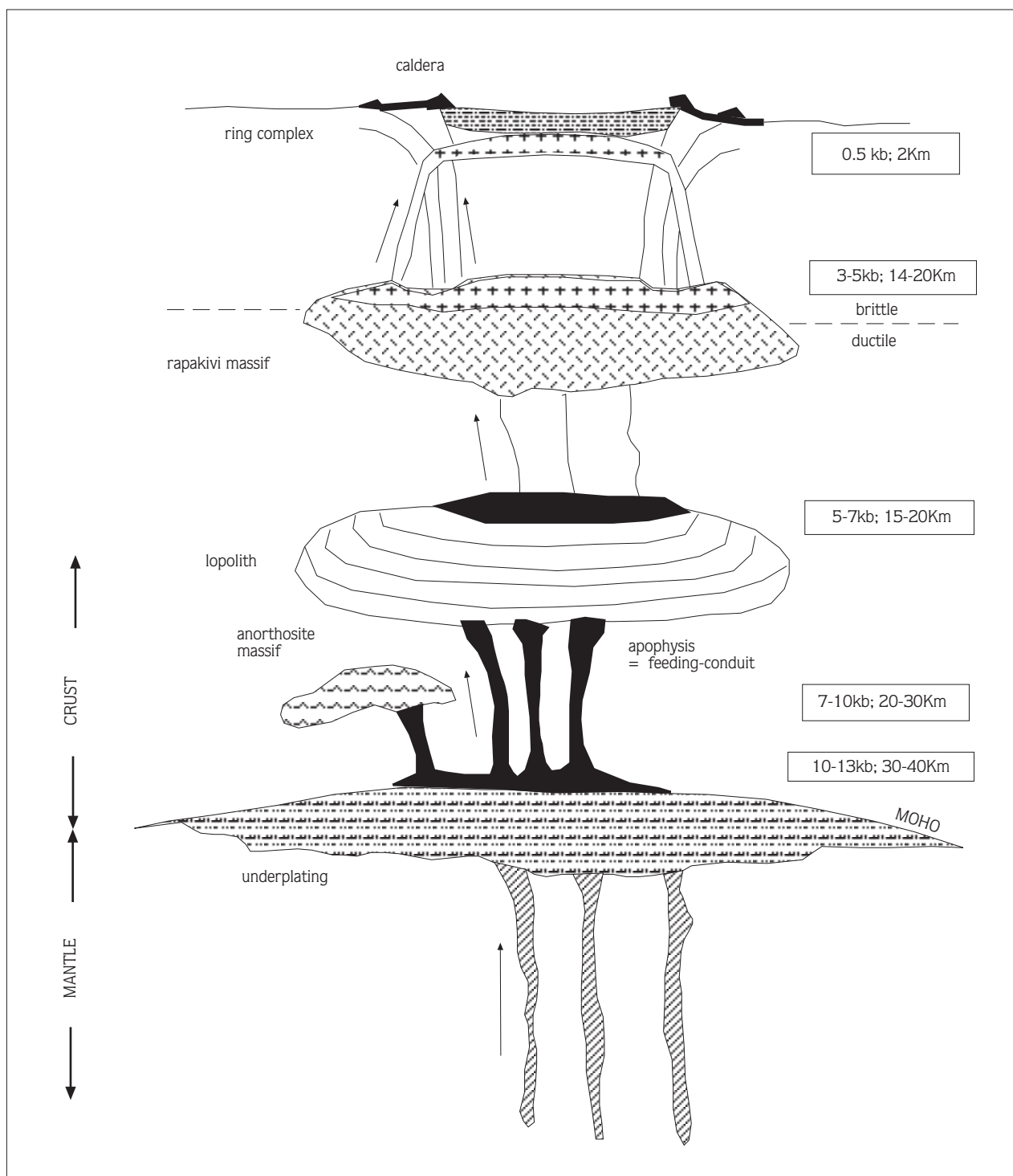
Figure 3. Structural levels of alkaline magmatism (Bonin, 1996): 1. Surface level: caldera volcano; 2. Subvolcanic level (1 to 4 km depth): ring complex, cone sheets and dyke swarms; 3. Magma chamber levels (14 to 30 km depth), from bottom to top: apophyses (black), anorthosite massif, mafic layered lopolith, rapakivi granite massif with alkali feldspar cumulates (dashes) and granitic residual liquids (crosses), 4. Crust-mantle boundary: storage of primary magmas formed within deeper asthenosphere. Though inappropriate (“intraplating” would be more adequate), “underplating” is maintained, because no other word has replaced it formally.
