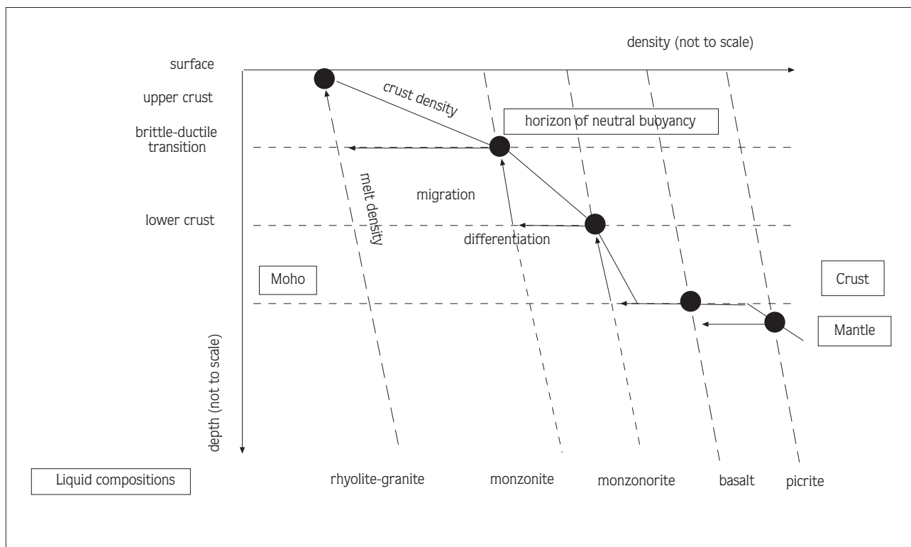
Figure 1. Density versus depth within crust and upper mantle. Each liquid of specific composition is capable to migrate upwards to its horizon of neutral buoyancy, where it is stored within a magma chamber and differentiates into a lighter more evolved residual liquid. The residual liquid can in turn migrate upwards to its own horizon of neutral buoyancy. A liquid can erupt at the surface level only in case of extension-driven decompression and displacement along wide conduits open well below its horizon of neutral buoyancy.
