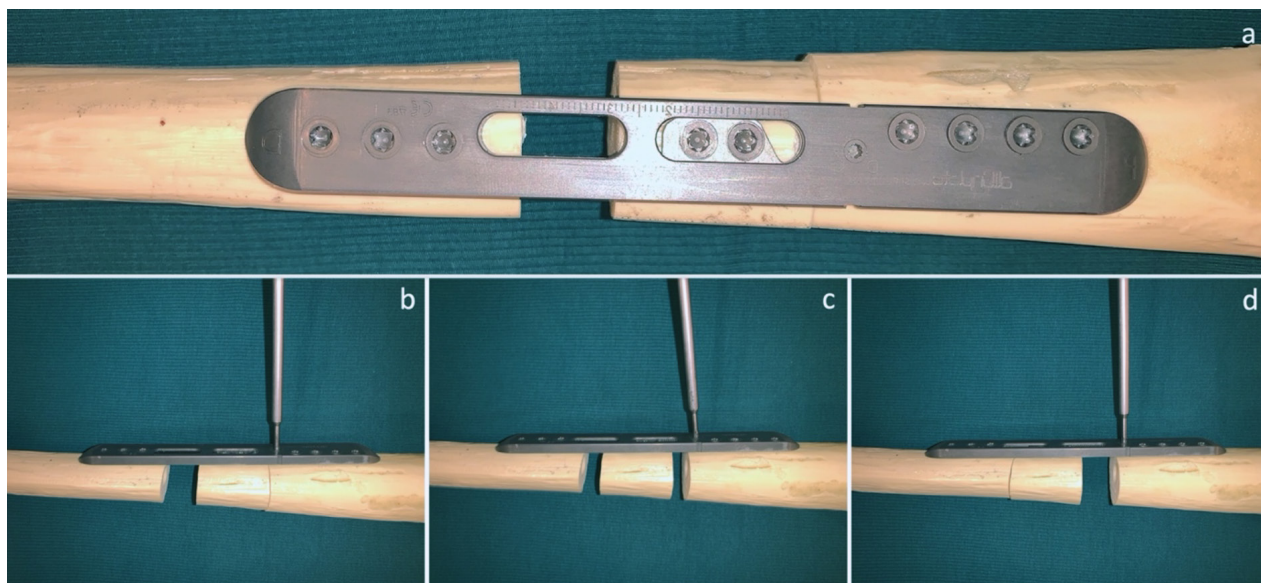
Figure 4. Fixation of ABP on sawbone with 15 mm bone defect model. (a) Top view, (b) Initial-stage of bone segment transfer, (c) Mid-stage of bone segment transfer, (d) End-stage of bone segment transfer.
