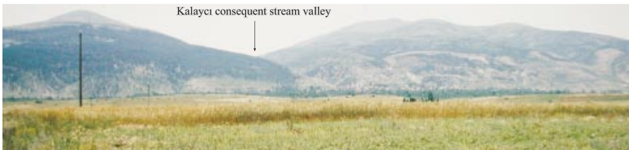
Figure 6. General view of the northward-facing scarp of the AkŐehir Fault Zone, which is transected and carved deeply by the Kalaycı consequent stream as a natural response to the active movement on the AkŐehir Master Fault (view towards south).
