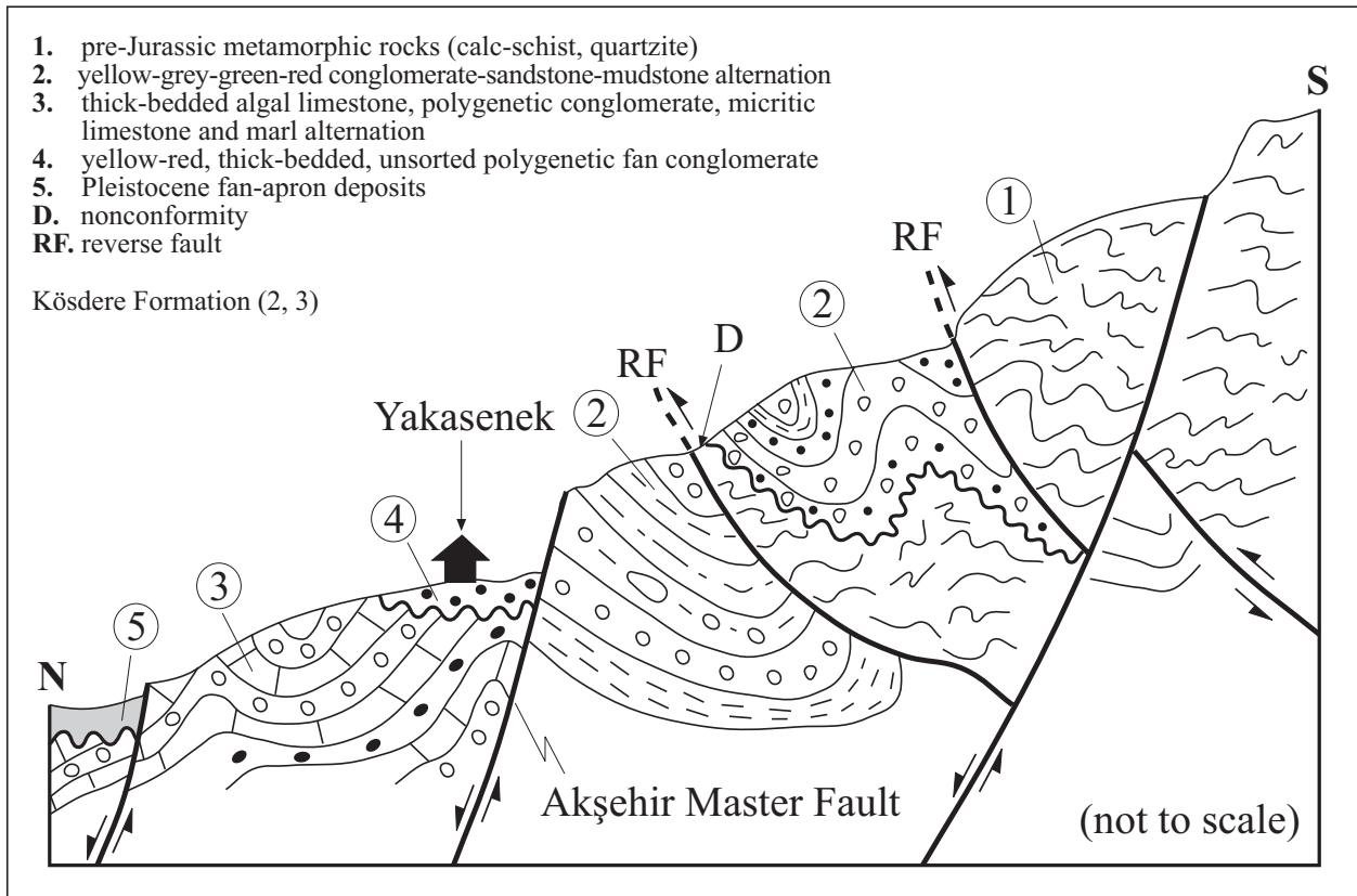
Figure 5. Sketched geological cross-section showing the folded and thrust faulted Köstere Formation (older infill) (see Figure 3 for location).
