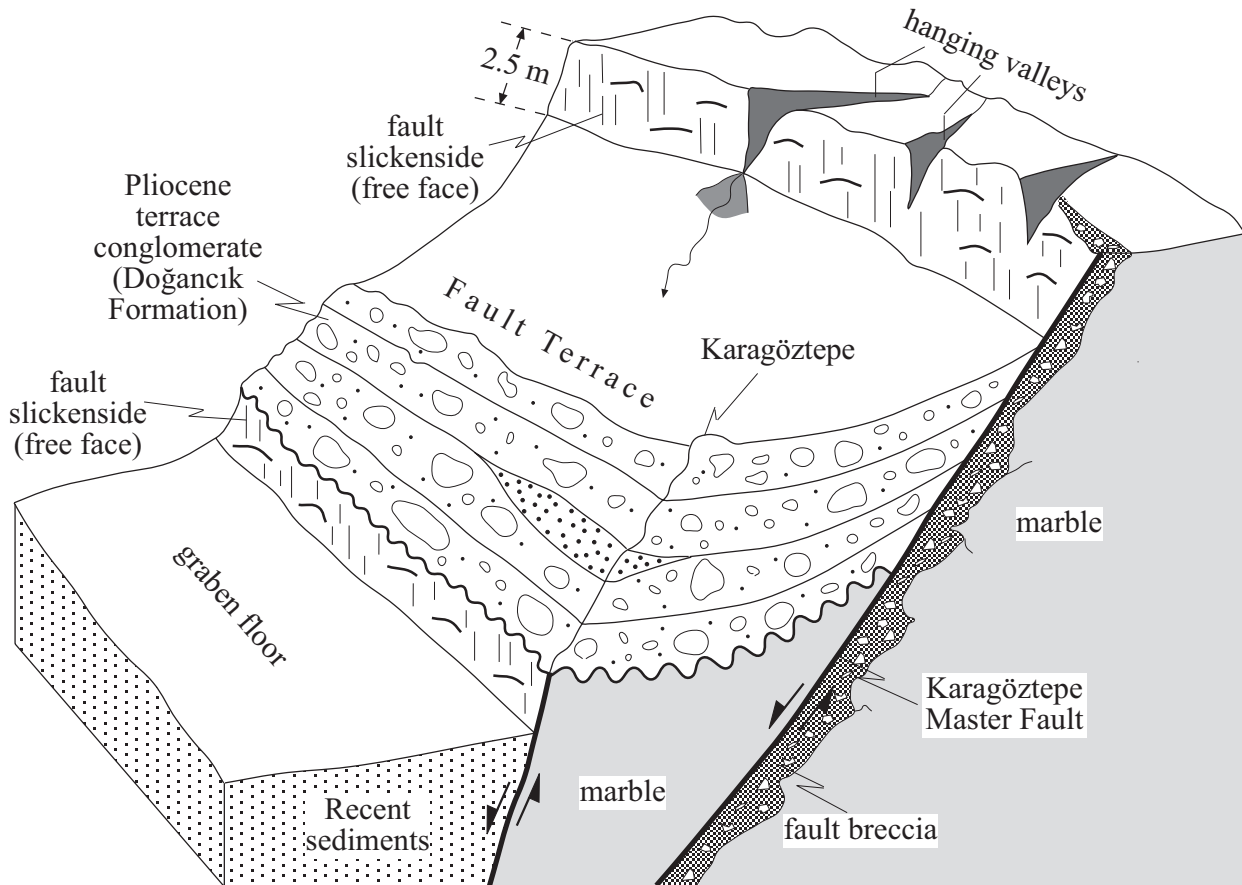
Figure 13. Sketched block diagram showing the well-preserved Karagöztepe Master Fault slickenside; faulted, terraced, uplifted (up to 200 m) and tilted Pliocene Doğancık Formation in the down-dropped southern block of the Karagöztepe Master Fault (see Figure 2 for location).
