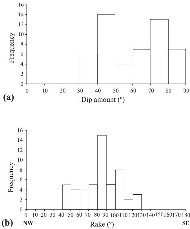
Figure 9. Histograms showing predominant dip and rake values of the Akşehir Master Fault.
