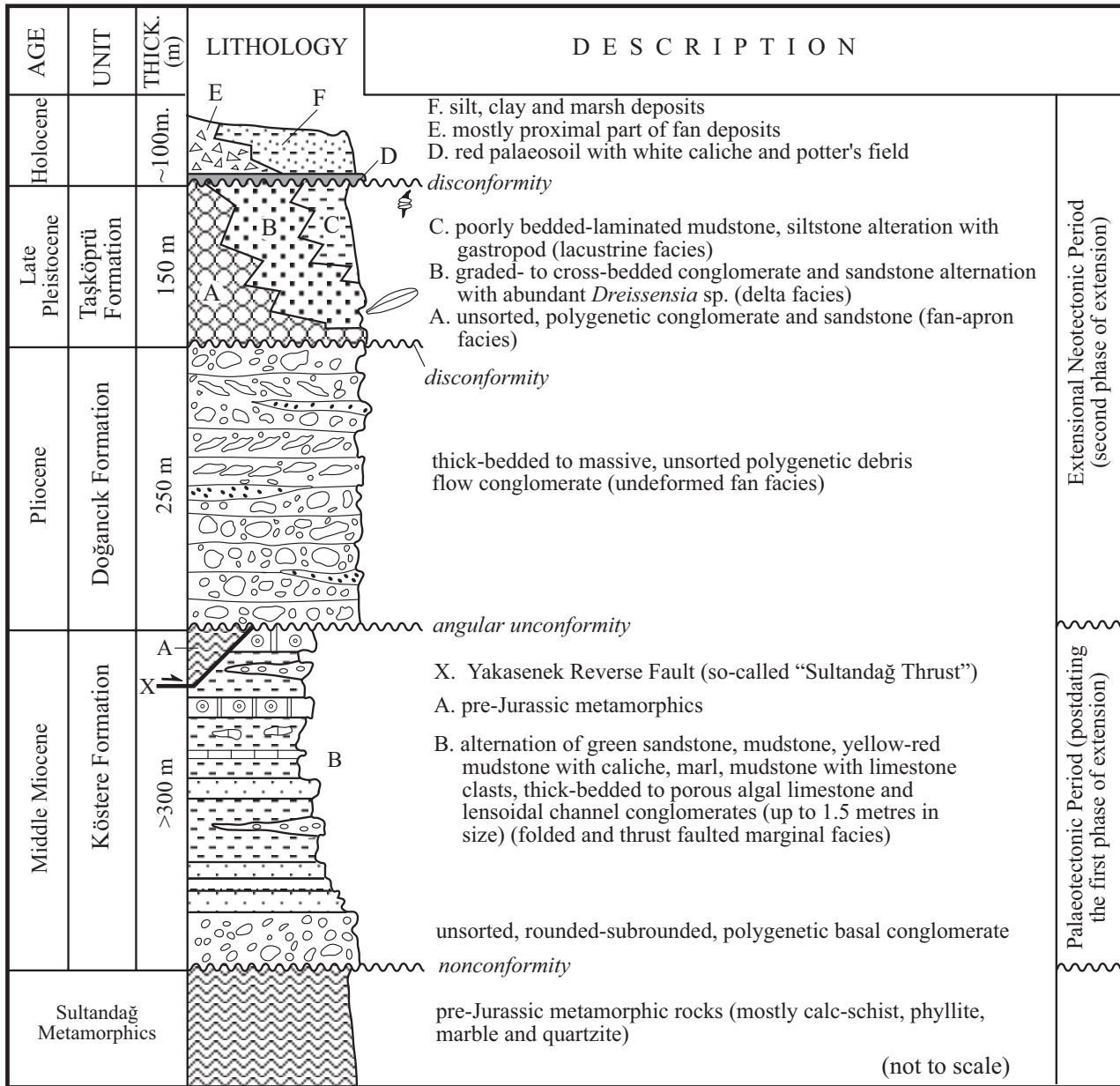
Figure 4. Generalised stratigraphical column of the graben fill (Yakasenek-Eber section of the Akşehir-Afyon Graben).
