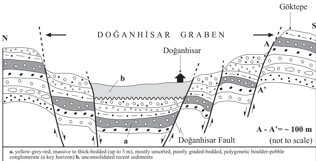
Figure 10. Sketched geological cross-section showing a small graben (Doğanhisar graben) bounded by step-like oblique-slip normal faults comprising the eastern section of the Akşehir Fault Zone. Yellow-red clastic rocks of the Pliocene Doğançık Formation are cut, terraced and displaced up to 100 m (A-A') by these faults (see Figure 2 for location).
