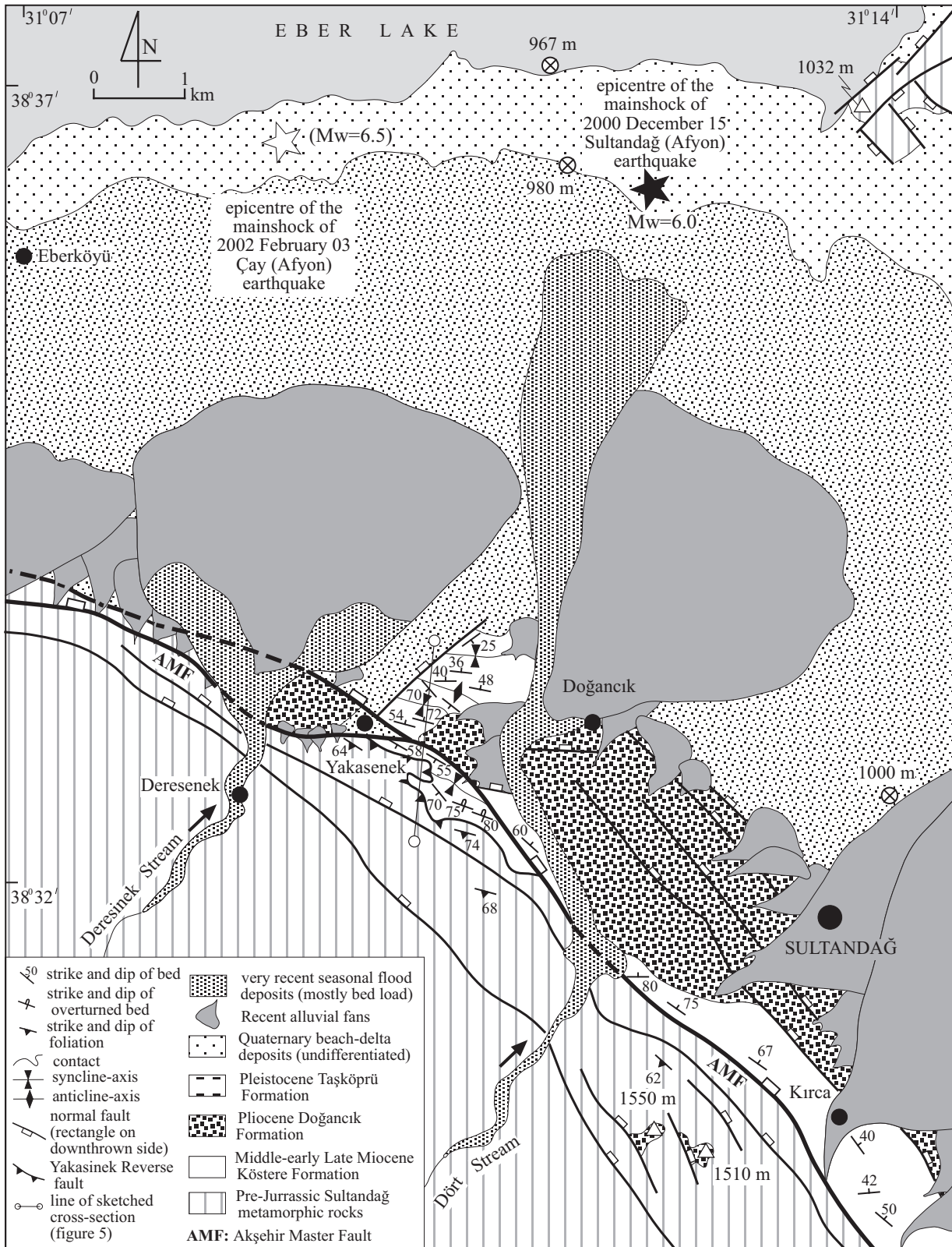
Figure 3. Geologic map of the Yakasenek-Eber section of the Akşehir-Afyon Graben (modified from Koçyiğit et al. 2000b).
