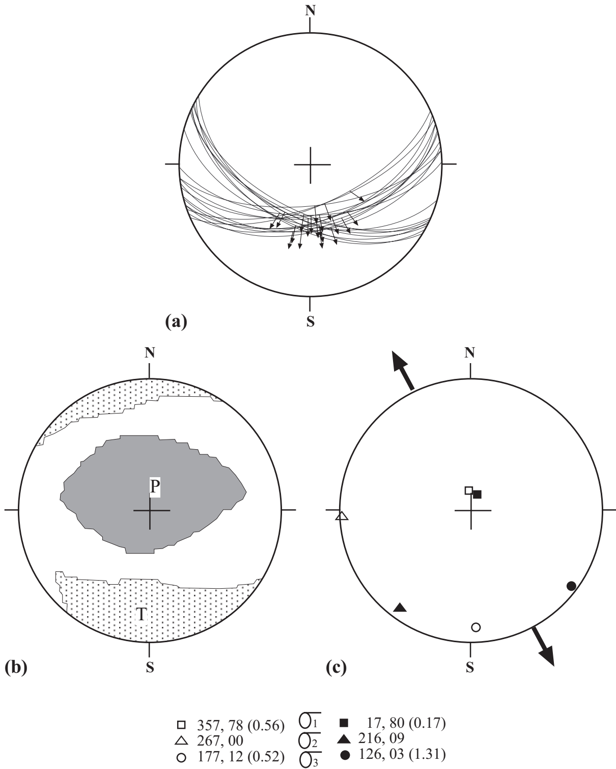
Figure 12. (a) Stereographic plots of the Karagöztepe Master Fault slip data on a Schmidt lower hemisphere net. (b) compression (P) and extension (T) diagram of the same data, and (c) diagram showing orientations of stress axes and the extension direction (arrows).
