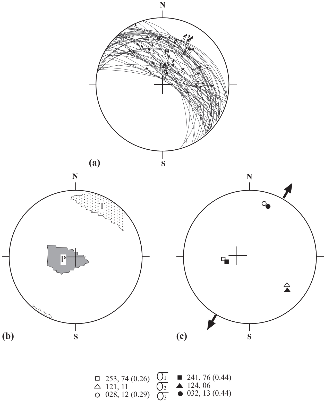
Figure 8. (a) Stereographic plots of the Akşehir Master Fault slip data on a Schmidt lower hemisphere net. (b) compression (P), and (c) diagram showing orientations of stress axes and the extension direction (arrows).
