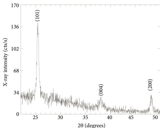
Figure 1. GIXRD spectra of \text{TiO}_2 -coated glass substrate after heat treatment at 500^\circ\text{C} .
