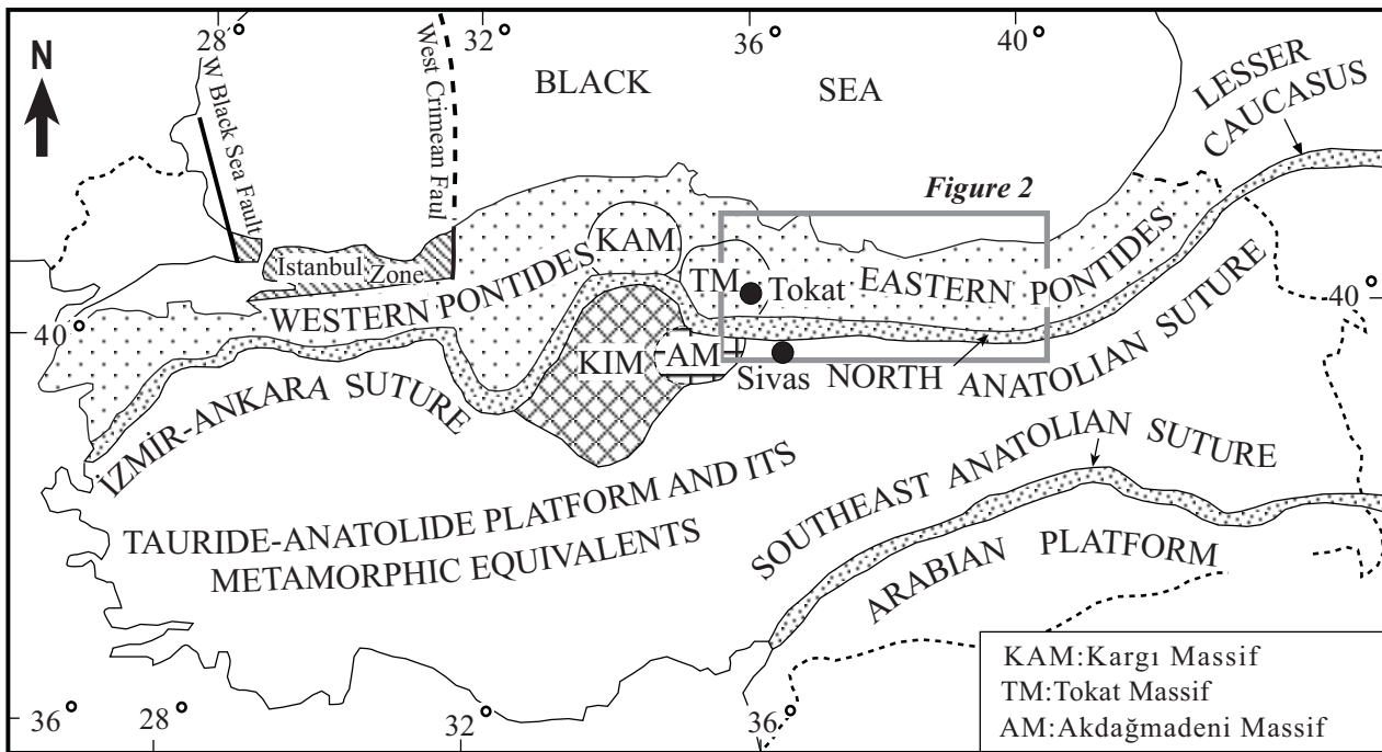
Figure 1. Simplified tectonic divisions of Turkey. The Pontides (shaded region) (after Ketin 1966 and general evaluations). Abbreviations: KAM–Kargı Massif, TM– Tokat Massif, AM– Akdağmadeni Massif. Inset shows the location of the map displayed in Figure 2 (after Okay 1989; Okay & Tüysüz 1999 and personal evaluations).
