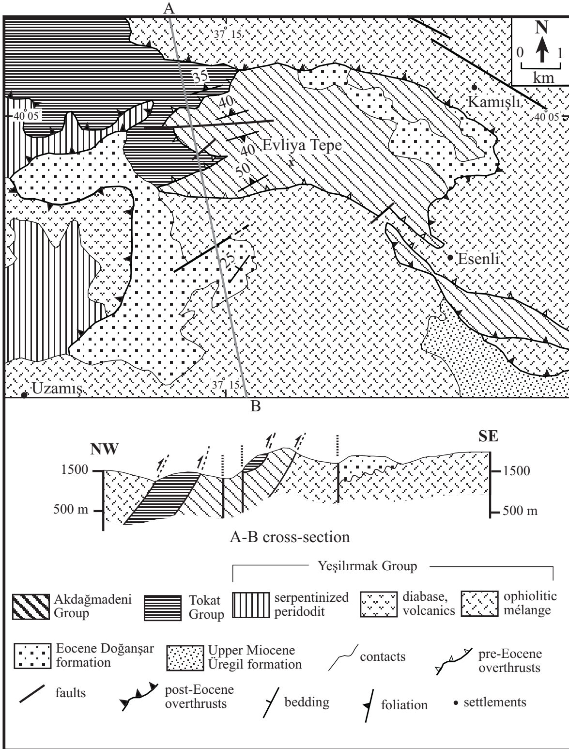
Figure 6. Geological map of the Evliya Tepe area showing relationship between Tokat Group, Akdağmadeni Group and Yeşilirmak Group (after A. Yılmaz 1982b). For location see Figure 2.
