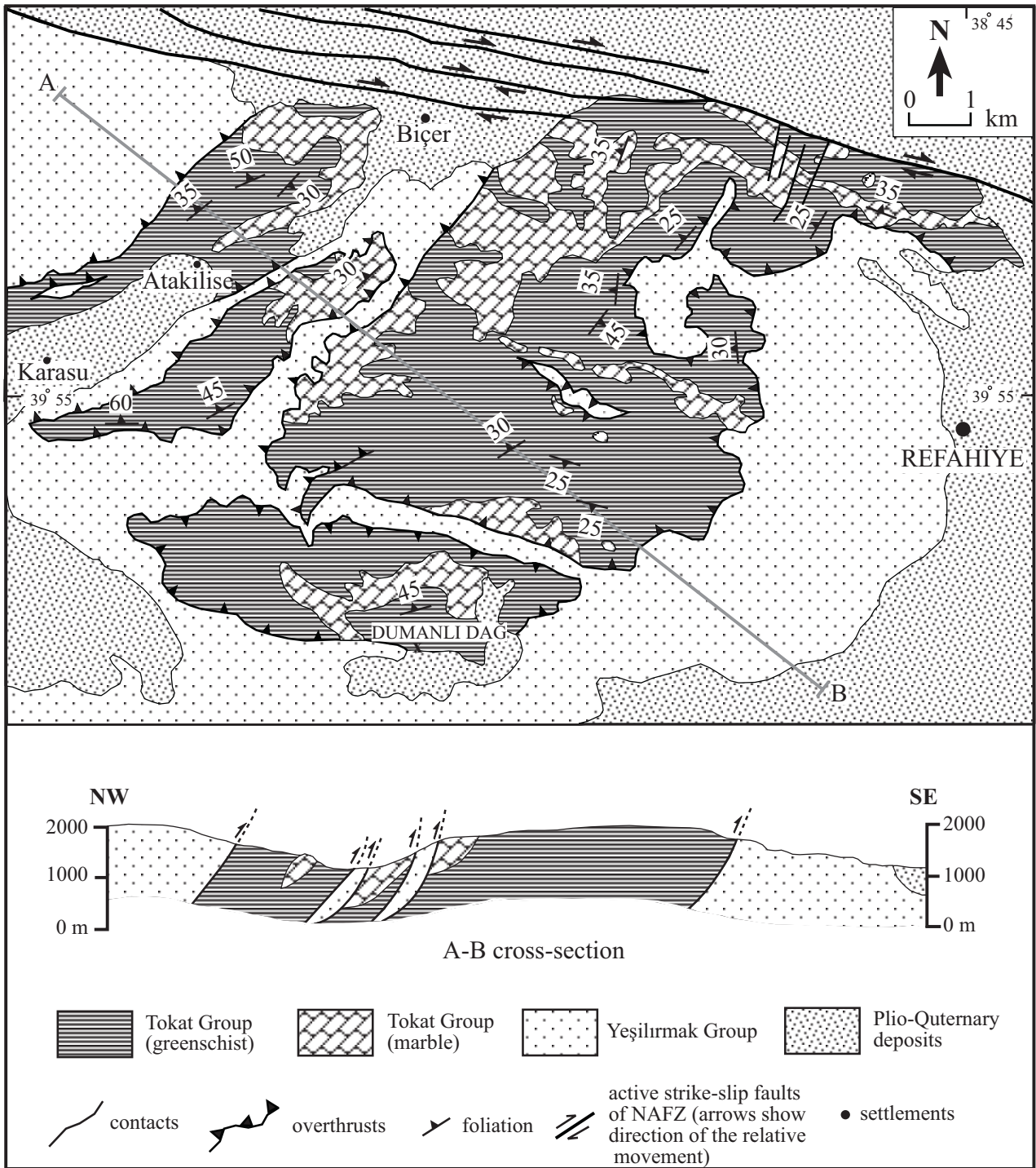
Figure 5. Geological map of Dumanlı Dağ of Refahiye area (after A. Yılmaz et al. 1985b). For location see Figure 2.
