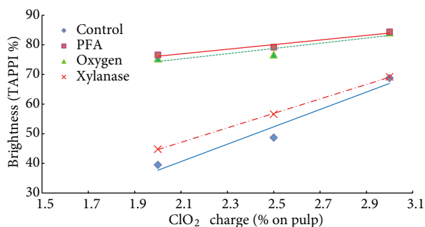
Figure 2. Effect of ClO 2 charge on the final brightness of bamboo pulp.
