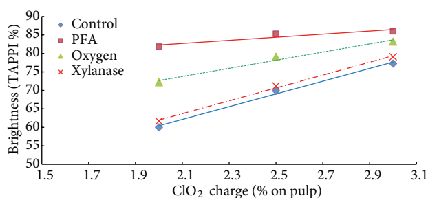
Figure 1. Effect of ClO 2 charge on the final brightness of hardwood pulp.
