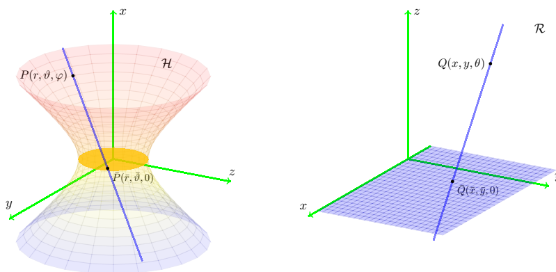
Figure. The hyperboloid and the right half-space models of \widetilde{SL(2, \mathbb{R})} geometry.
