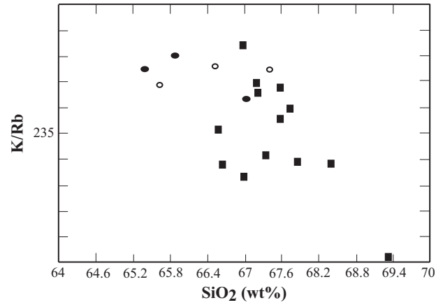
Figure 2. SiO_2 versus K/Rb diagram (after Wyborn 1992). (■: granodiorite; ◆: quartz-monzodiorite; ○: quartz-diorite).
