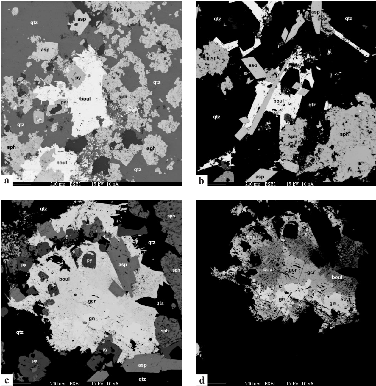
Figure 2. (a) A backscatter image from section idg2 showing an anhedra grain of boulangerite (boul) with euhedral grains of pyrite (py) and arsenopyrite (asp), and anhedral grains of sphalerite (sph), all embedded in a matrix of quartz (qtz). (b) A backscatter image from section idg1 centred on a grain of boulangerite (boul) surrounded by euhedral grains of arsenopyrite (asp) and anhedral grains of sphalerite (sph), all embedded in a matrix of quartz (qtz). (c) A backscatter image from section idg2 centred on an anhedra grain of galena (gn) with geocronite (gcr), and boulangerite (boul), accompanied by euhedral grains of pyrite (py) and arsenopyrite (asp), and anhedral grains of sphalerite (sph), enmeshed in a matrix of quartz (qtz). (d) An enhanced backscatter image of an anhedra grain in (c) of galena (gn), geocronite (gcr) and boulangerite (boul). Note the decrease in brightness with decreasing content of Pb as one progresses from the core of galena through the overgrowth of geocronite to the outer rim of boulangerite.
