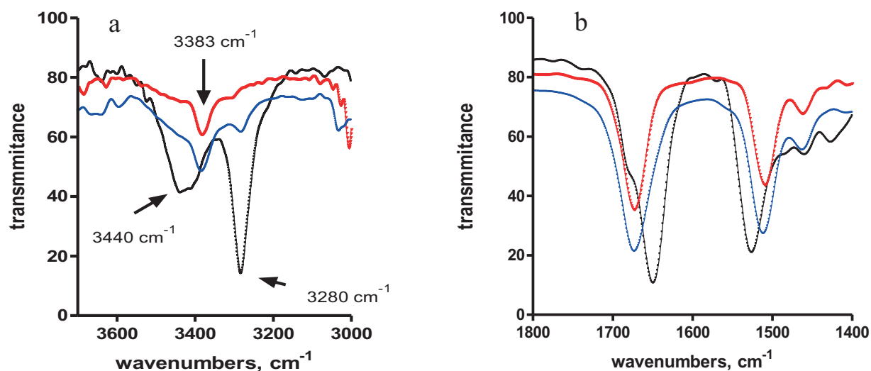
Figure 7. FTIR spectra of 4 in the xerogel form from xylene gel and in the solution diluted by chloroform. (a) 3500–3000 \text{cm}^{-1} , (b) 1800–1400 \text{cm}^{-1} .
