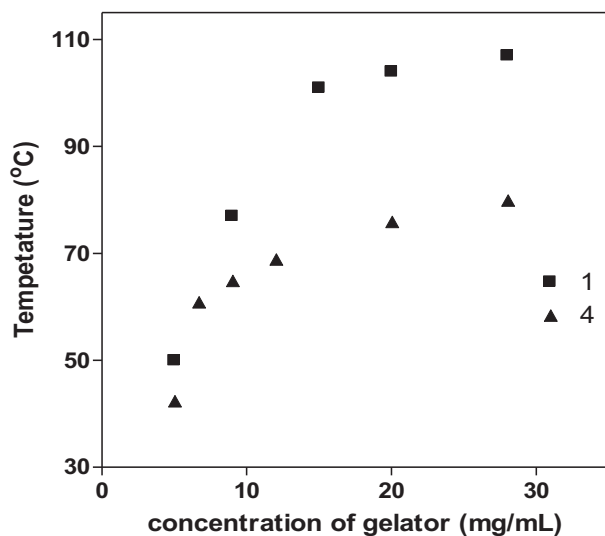
Figure 4. A plot of the gel-to-sol transition temperature ( T_{gel} ) against the concentration of the gelators (1 and 4) in PhEME.
