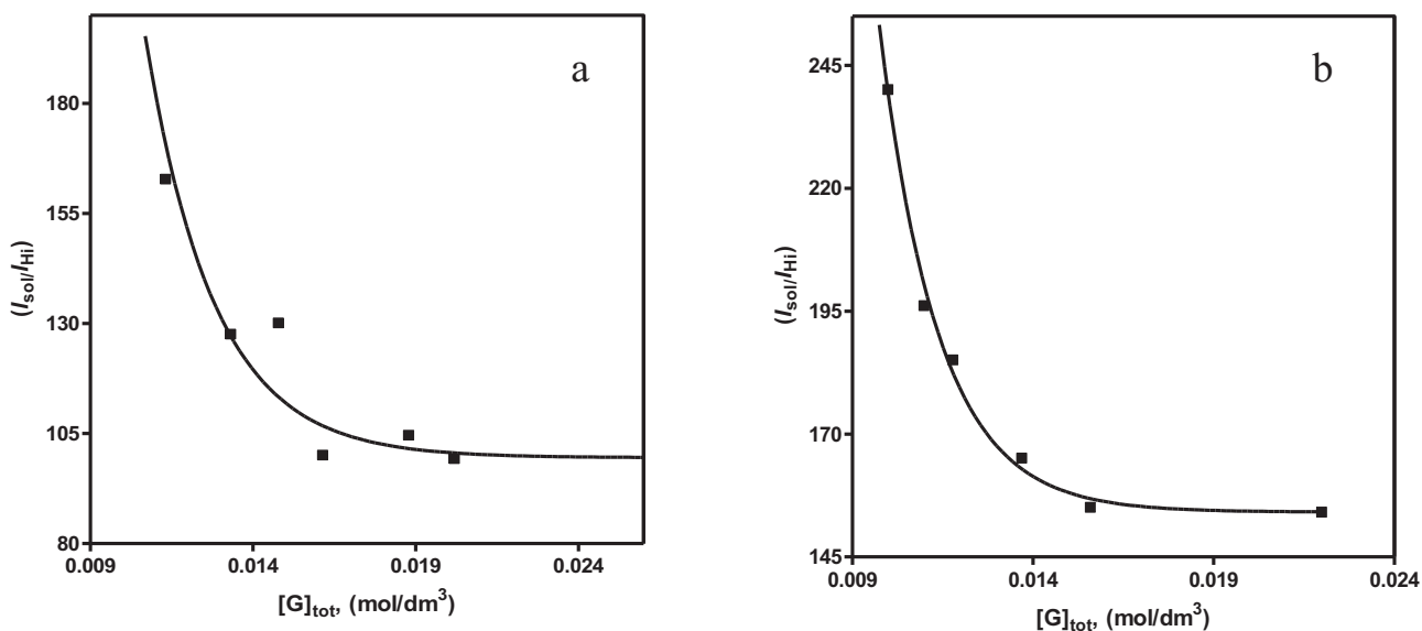
Figure 9. The plot of I_{sol}/I_{Hi} against the concentration of the gelator for the gelators: (a) 1 in \text{CD}_3\text{CN} and (b) 4 toluene- d_8 .
