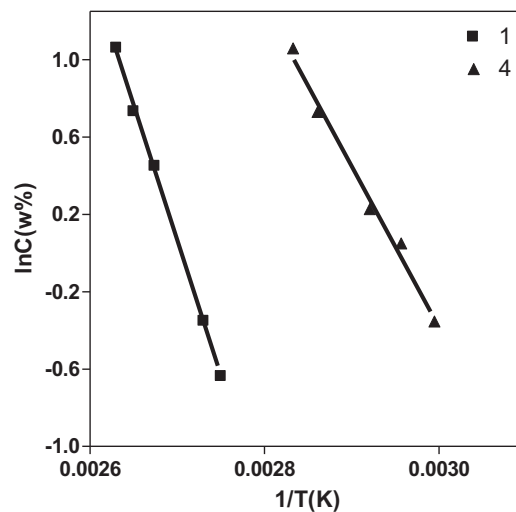
Figure 5. van't Hoff plot of 1 and 4 gelators in PhEME.
