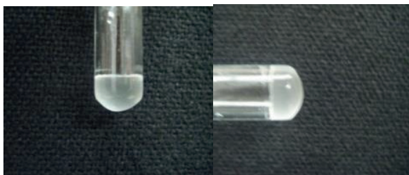
Figure 1. A typical gel structure of 4 in xylene.
