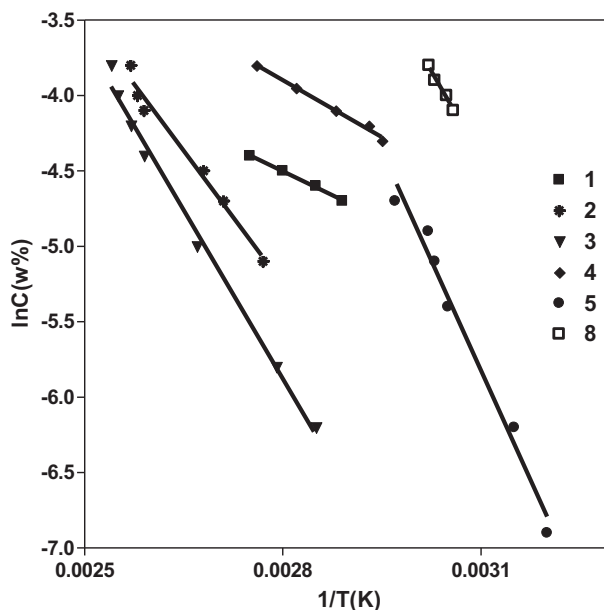
Figure 3. van't Hoff plot of gelators 1 , 2 , 3 , 4 , 5 , and 8 in anisole.
