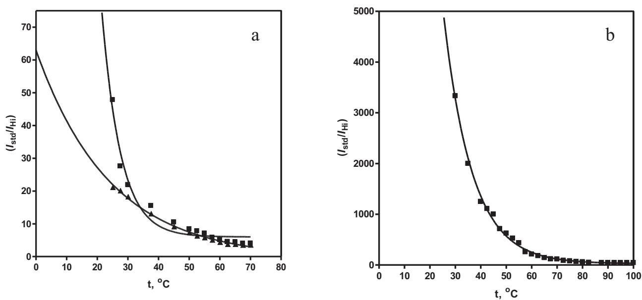
Figure 8. The plot of I_{std}/I_{Hi} against temperatures for the gelators: (a) 1 in \text{CD}_3\text{CN} where solid squares correspond to the integration in ^*\text{CH} and angles to that in \text{NH} and (b) 4 in toluene- d_8 involving the internal standard ( \text{Cl}_2\text{CHCHCl}_2 ).
