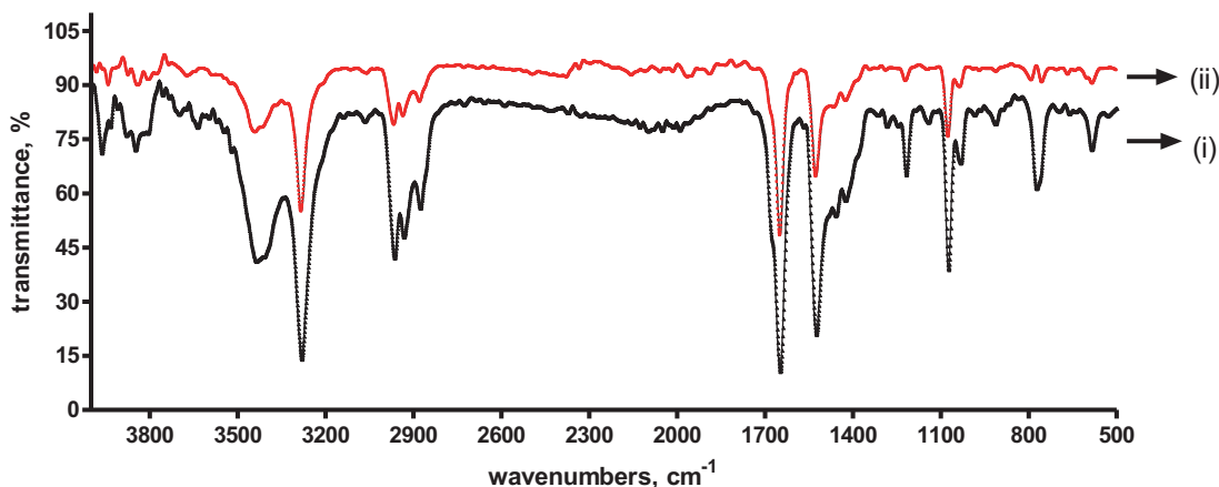
Figure 6. FTIR spectra of 4 in the solid state and the xerogel form from xylene gel.
