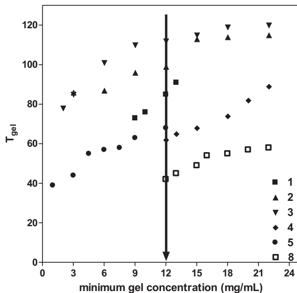
Figure 2. A plot of gel-to-sol transition temperature ( T_{gel} ) against the minimum gel concentration (mg/mL) of gelators 1 , 2 , 3 , 4 , 5 , and 8 in anisole.
