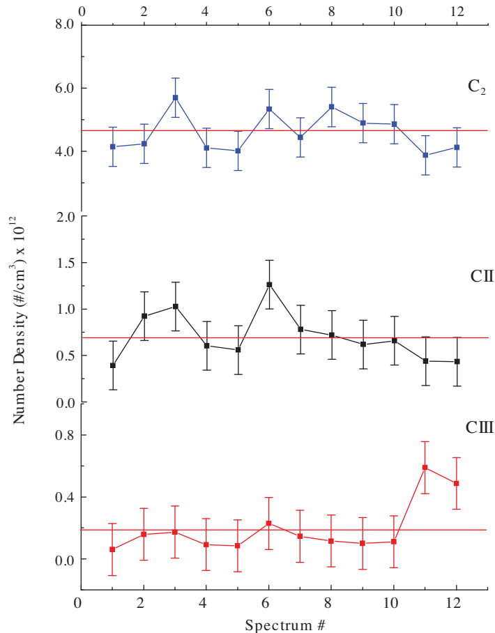
Figure 5. Intensities of \text{C}_2 , CII and CIII plotted for set of pulsed arc discharge experiments.
