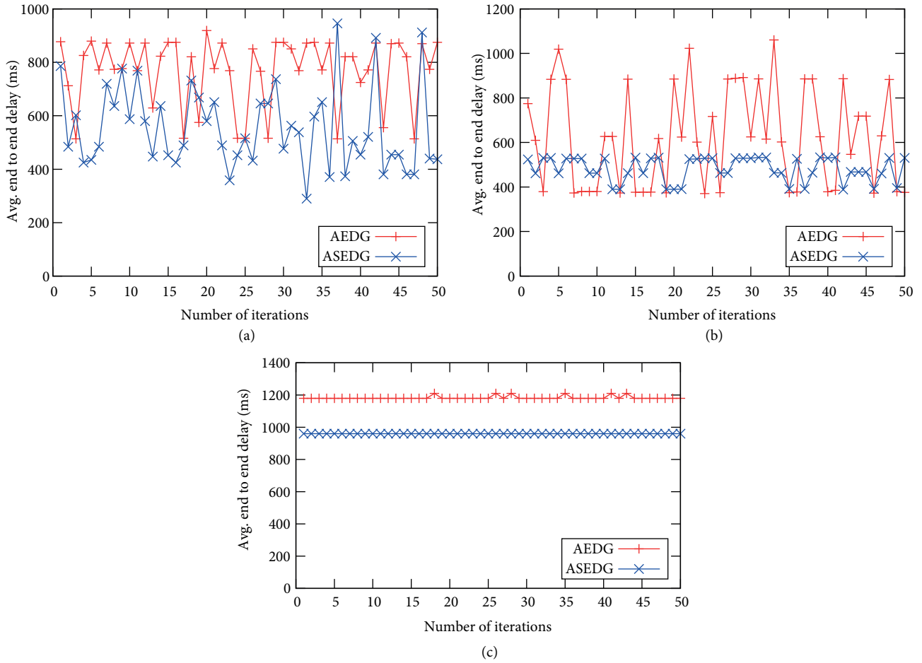
Figure 7. Average end-to-end delay of 100 static nodes in (a) 500 m × 500 m, (b) 1000 m × 1000 m, (c) 1500 m × 1500 m.
