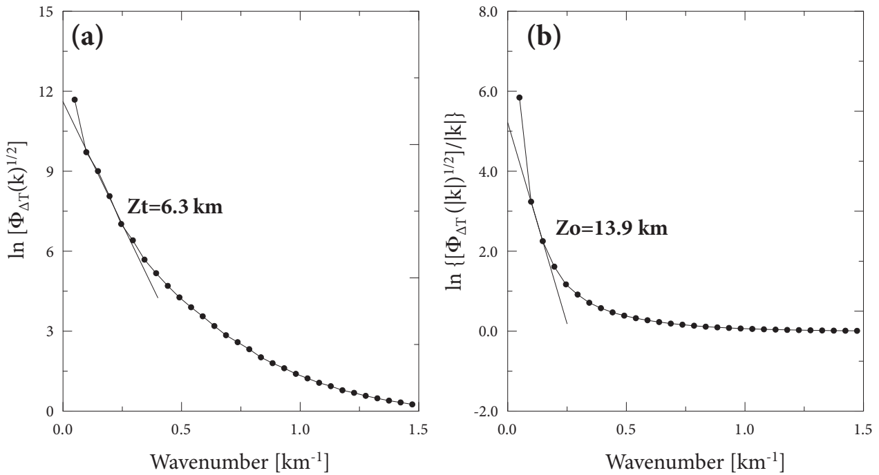
Figure 5. Examples of spectra for the estimation of the depth to Curie point using the 2D magnetic anomaly data covering a region of (35°E, 41°N)–(36°E, 42°N). The values over the linear segments are the depths to the upper limit ( Z_t = 6.3 \text{ km} ) and centroid ( Z_o = 13.9 \text{ km} ) estimated by the least squares method.
