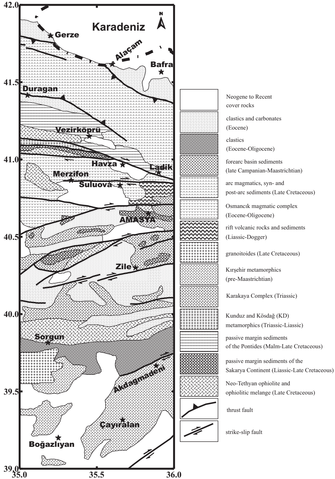
Figure 2. Geological map of the Central Pontides (modified from Yılmaz et al. 1997).
