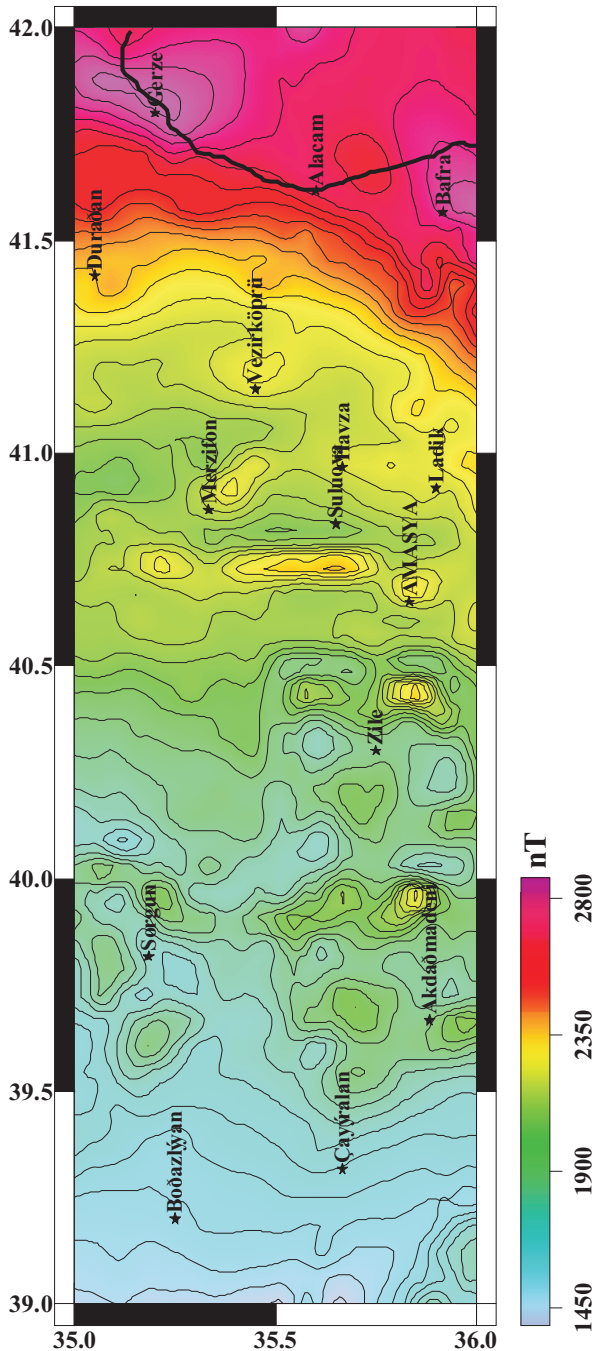
Figure 3. Magnetic anomaly map of the study region. Contour interval is 50 nT. Colour bar indicates interval values. Colour levels point out anomaly intensity from magenta (highest) to blue (lowest).
