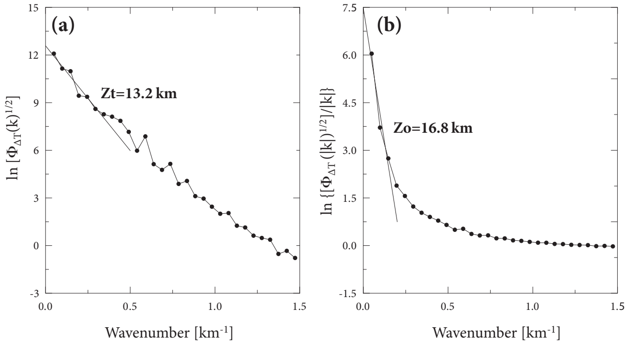
Figure 4. The Power spectrum curves of the reduced to pole magnetic data of the study region. The values over the linear segments are the depths to the upper bound ( Z_t = 13.2 \text{ km} ), and centroid ( Z_o = 16.8 \text{ km} ) estimated by least squares method.
