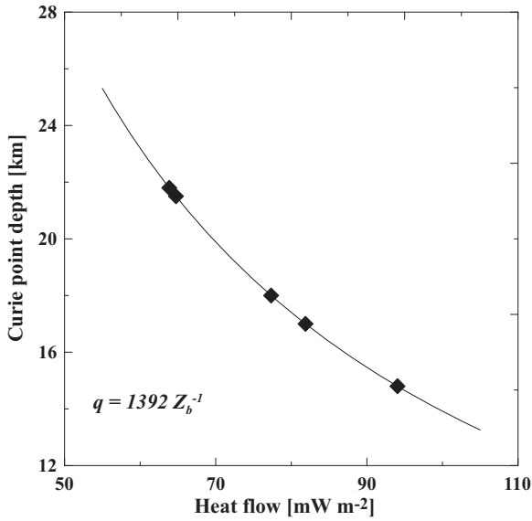
Figure 7. The Curie point depth versus heat flow data graph for the study region.
