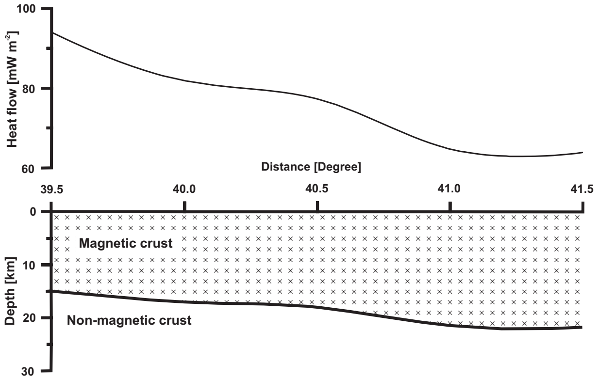
Figure 6. 2D Curie point depth and heat flow anomaly section for the study region.
