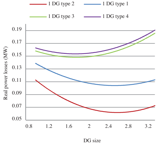
Figure 5. Effect of DG size variation on active power losses.
