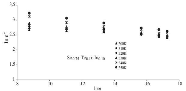
Figure 9. \ln \omega vs \ln \epsilon'' curves in a- \text{Se}_{0.75}\text{Te}_{0.15}\text{In}_{0.10} at certain fixed temperatures.
