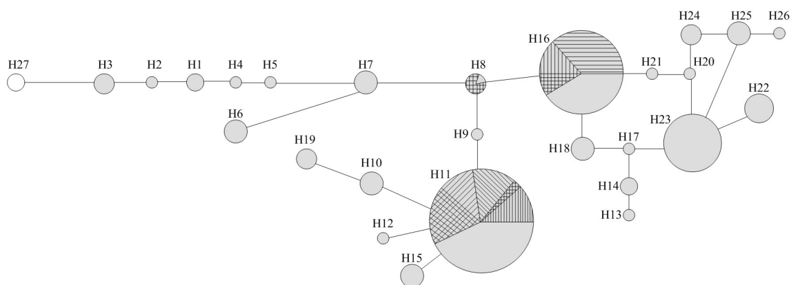
Figure. Network representation of the haplotypes identified in six cattle breeds reared in Poland and in Rathi cattle. The haplotypes of Kantanen et al. (2009) were used as reference. The circle size is proportional to the haplotype frequency. Breed groups are represented as follows: PR (vertical), PW (cross), PRW (backward diagonal), PBW (forward diagonal), PHF (diagonal cross), SIM (horizontal), Rathi (solid white), and reference haplotypes (solid gray).
