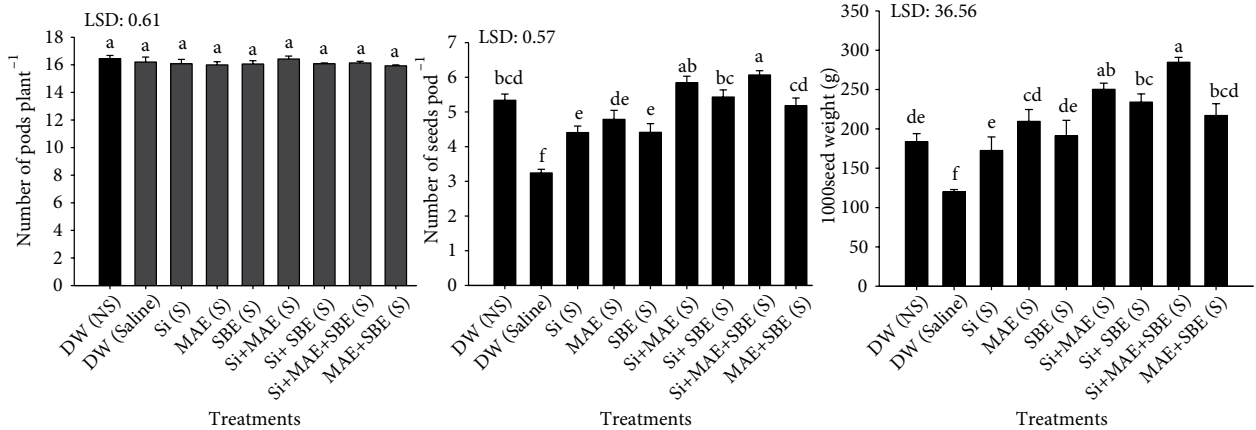
Figure 6. Effect of phyto-extracts (MAE and SBE) and Si on yield attributes of salt-stressed pea plants. Each value represents the mean of 5 replicates ± standard error (SE) of the mean. Letters represent mean separation comparison utilizing least significant difference (LSD) test ( P \geq 0.05 ) (Si: silicon, MAE: Melia azedartha leaf extract, SBE: sugar beet root extract).
