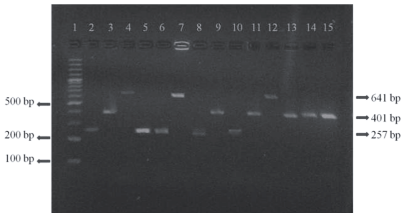
Figure. Gel electrophoresis image of m-PCR for Arcobacter species isolated from cloacal swab and feces samples of geese. 1: DNA marker (Gene ruler 100 bp DNA Ladder, Fermentas); 2: positive control, A. cryaerophilus (257 bp); 3: positive control, A. butzleri (401 bp); 4: positive control, A. skirrowii (641 bp); 5–13: isolates of cloacal swab; 14–15: isolates of feces.
