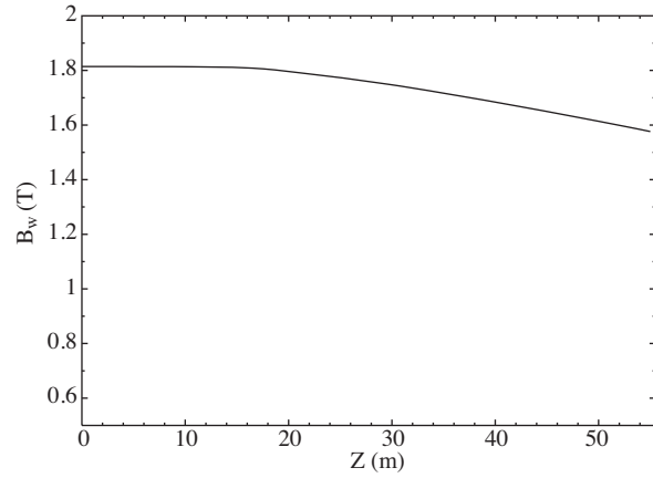
Figure 5. Magnetic field on the wiggler axis vs wiggler length.
