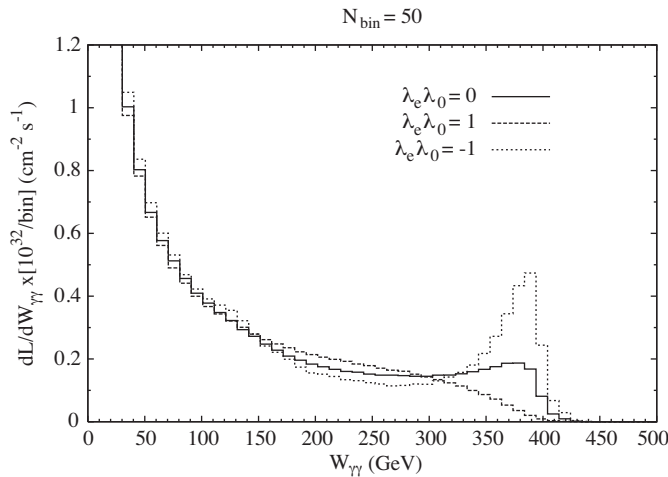
Figure 2. CLIC \gamma\gamma Luminosity spectra at E_{\text{cm}} = 0.5 TeV for different helicity states of electron ( \lambda_e ) and FEL photons ( \lambda_0 ).
