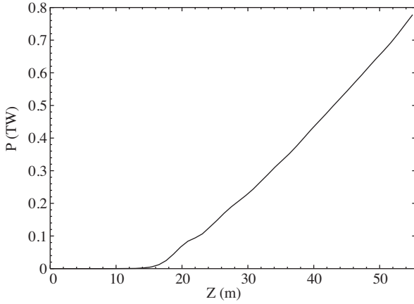
Figure 4. FEL Power as a function of wiggler length.
