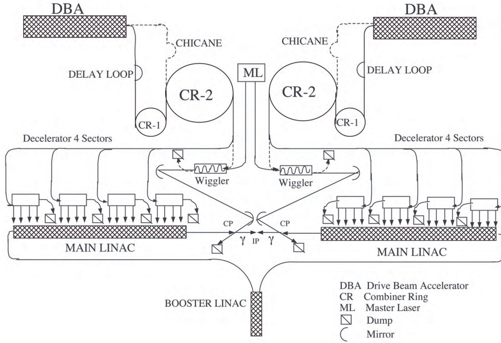
Figure 3. Layout of CLIC \gamma\gamma collider and proposed laser system. Dashed line shows short train of the drive beam.
