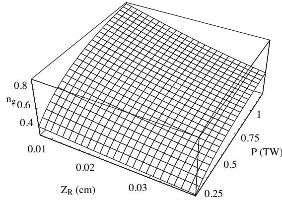
Figure 1. Conversion efficiency vs Z_R and peak power at A = 2 J
