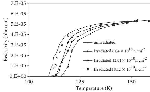
Figure 1. Temperature dependence of resistivity for Tl_{0.6}Pb_{0.3}Cd_{0.1}Ba_2Ca_2Cu_3O_{9-\delta} samples.
