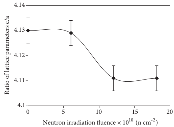
Figure 4. Ratio of lattice parameters c/a as a function of neutron irradiation fluence for Tl 0.6 Pb 0.3 Cd 0.1 Ba 2 Ca 2 Cu 3 O 9-δ samples.
