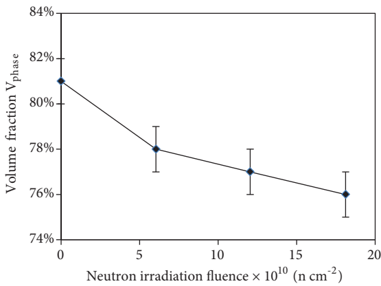
Figure 3. Volume fraction V (phase) as a function of neutron irradiation fluence for Tl 0.6 Pb 0.3 Cd 0.1 Ba 2 Ca 2 Cu 3 O 9-δ samples.
