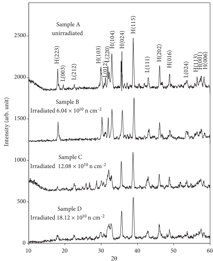
Figure 2. XRD patterns for the Tl_{0.6}Pb_{0.3}Cd_{0.1}Ba_2Ca_2Cu_3O_{9-\delta} samples.
