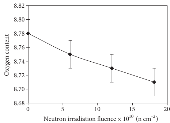
Figure 5. Oxygen content as a function of neutron irradiation fluence for \text{Tl}_{0.6}\text{Pb}_{0.3}\text{Cd}_{0.1}\text{Ba}_2\text{Ca}_2\text{Cu}_3\text{O}_{9-\delta} samples.
