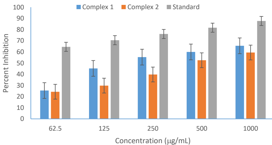
Figure 6. Graphical representation of percent inhibition of compounds 1 and 2 against ABTS, IC_{50} values are 165, 437, and 17.47 \mu\text{g/mL} for compounds 1 , 2 , and standard (gallic acid), respectively.
