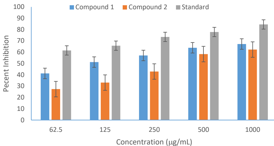
Figure 5. Graphical representation of percent inhibition of compounds 1 and 2 against DPPH, IC_{50} values are 114, 341, and 23.2 \mu\text{g/mL} for compounds 1 , 2 , and standard (gallic acid), respectively.
