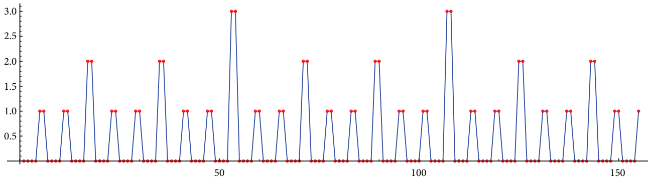
Figure 2. The 3-adic valuation of the Tripell numbers
