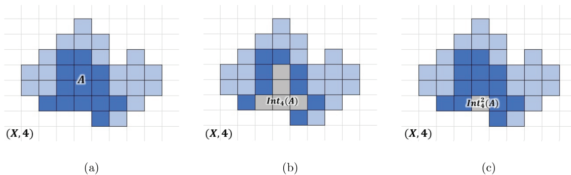
Figure 4. (a) Digital image (X, 4) , its subset A and (b) Int_4(A) , (c) Int_4^2(A) . Digital image X , A and interiors are shown in blue, dark blue and gray color, respectively.
