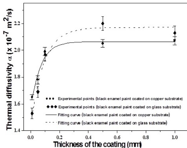
Figure 4. Variation in thermal diffusivity of dry black enamel paint coatings with thickness, coated on glass and copper substrates, and the corresponding fitting curves.
