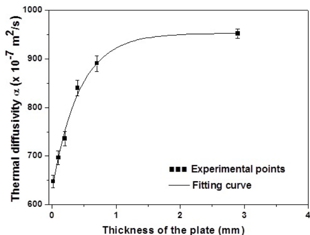
Figure 1. Variation in thermal diffusivity of thin free-standing copper plates with thickness, and the corresponding fitting curve. The two lowest thickness readings (0.02 mm and 0.1 mm) are for copper films coated on an insulating substrate (ebonite).
