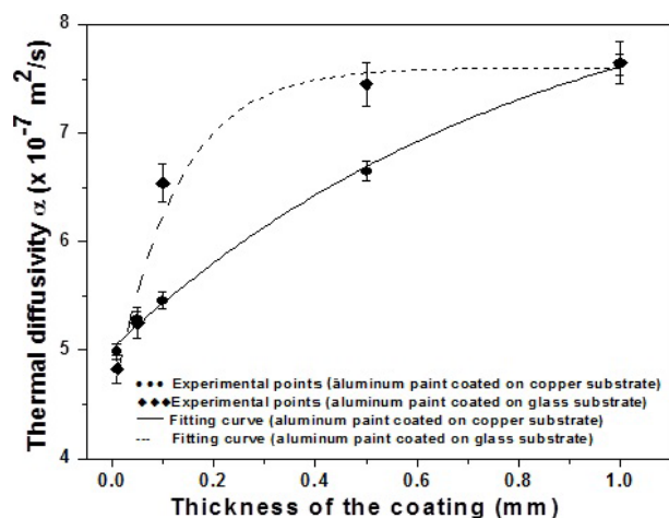
Figure 3. Variation in thermal diffusivity of dry aluminum paint coatings with thickness, coated on glass and copper substrates, and the corresponding fitting curves.
