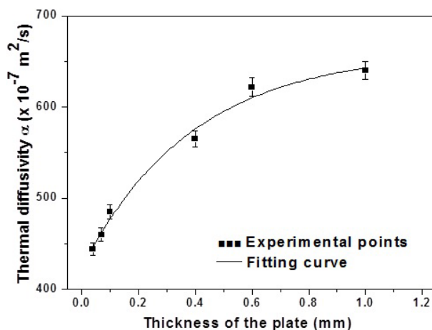
Figure 2. Variation in thermal diffusivity of free-standing aluminum plates with thickness, and the corresponding fitting curve.
