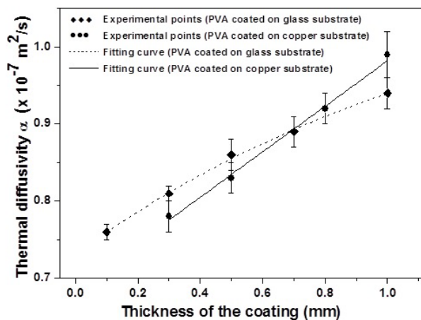
Figure 5. Variation in thermal diffusivity of PVA coatings with thickness, coated on glass and copper substrates, and the corresponding fitting curves.
