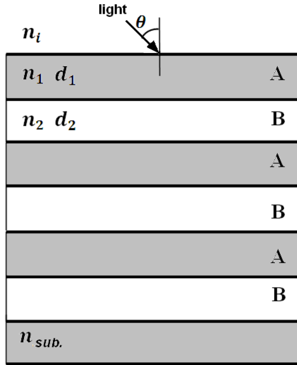
Figure 2. Schematic representation of a multilayered photonic crystal structure consisting of alternate layers.
