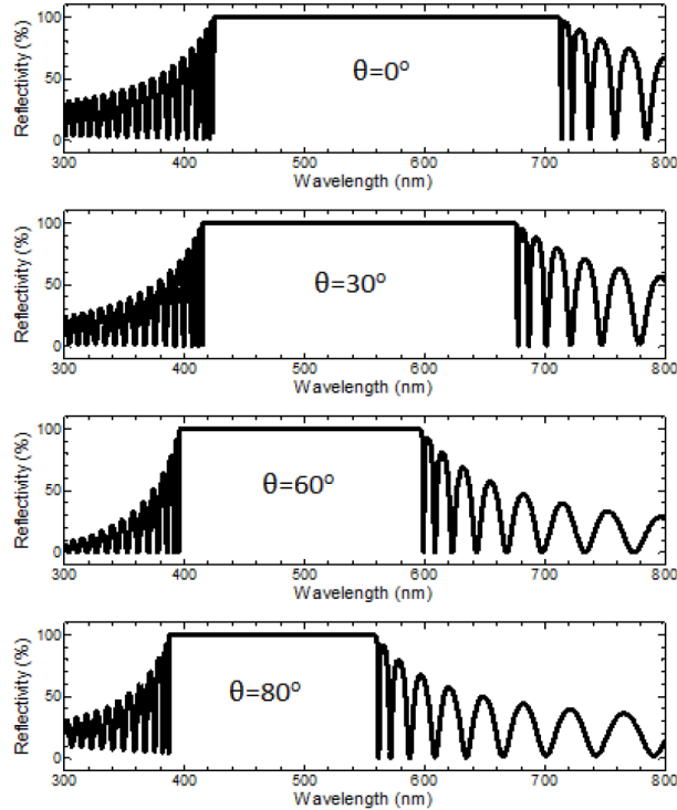
Figure 4. Reflectivity spectra of air/(AB) 24 /substrate and the different angles of incidence for TM polarization.
