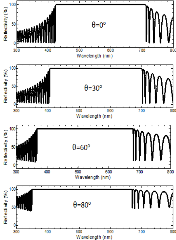
Figure 3. Reflectivity spectra of air/(AB) 24 /substrate and the different angles of incidence for TE polarization.
