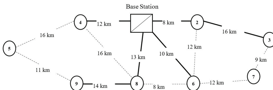
Figure 5. Single-line diagram of the IEEE standard 9-bus system.
