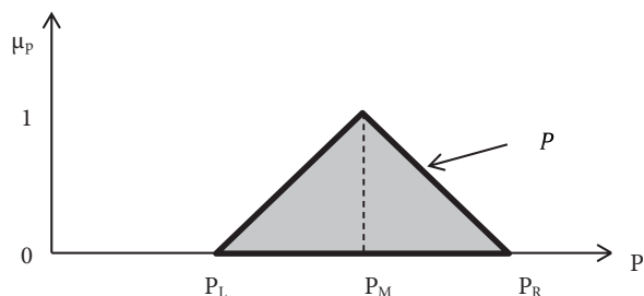
Figure 1. Graphical representation of the load as a triangular fuzzy number.
