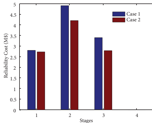
Figure 7. Comparison of customer outage cost during the years of planning horizon in the two scenarios.
