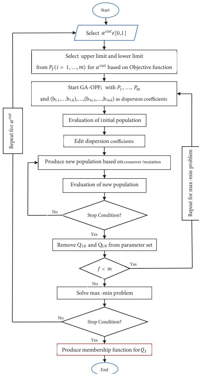
Figure 3. Process of modeling the uncertainties based on the fuzzy theory incorporation with GA-OPF algorithm.
