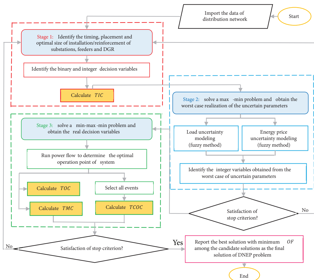
Figure 4. Flowchart of the proposed tri-stage decomposition approach for solving the DNEP problem.
