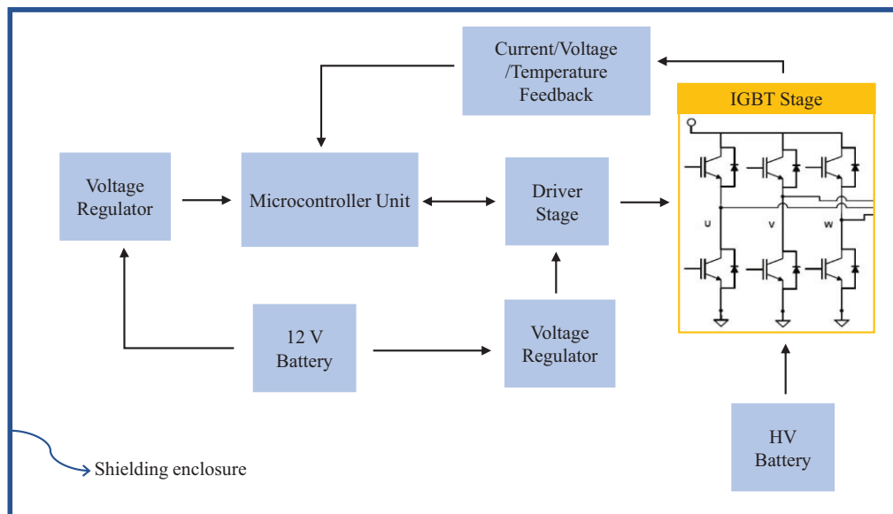
Figure 1. Inverter block diagram.
