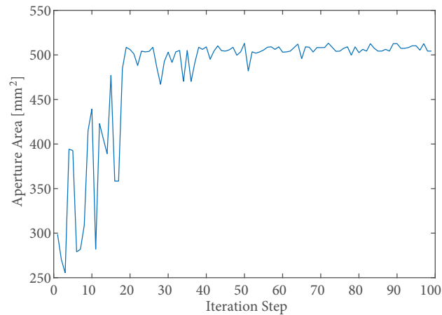
Figure 9. The change in aperture area for each iteration step of O3 result.
