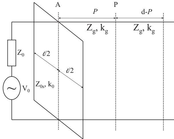
Figure 3. Equivalent circuit of the rectangular enclosure with an aperture.
