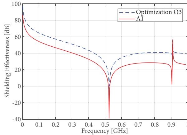
Figure 7. SE optimization result obtained by O3 .
