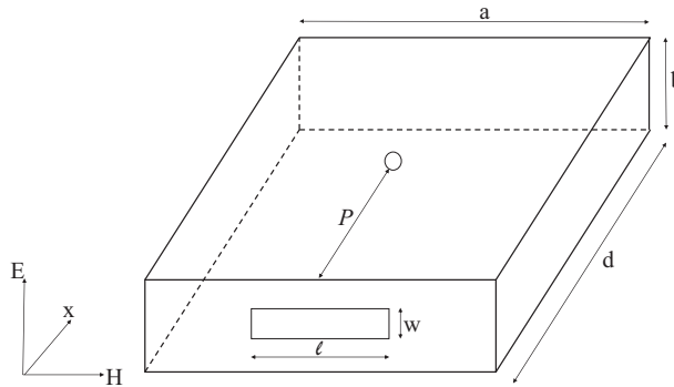
Figure 2. A rectangular enclosure with an aperture.
