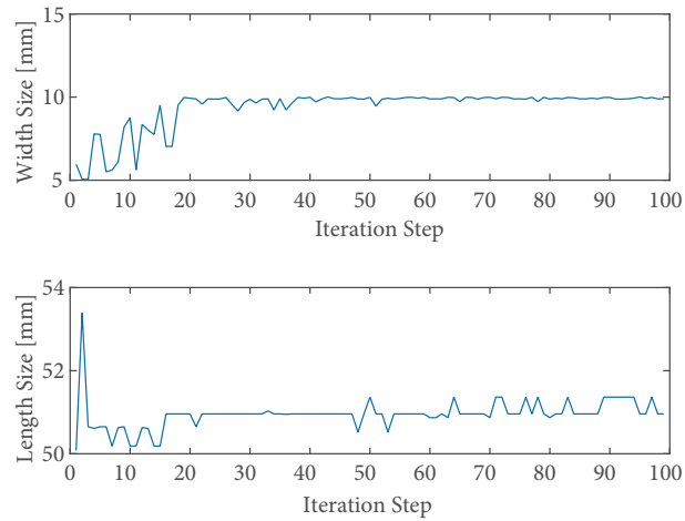
Figure 8. The change in aperture dimensions for each iteration step of O3 result.
