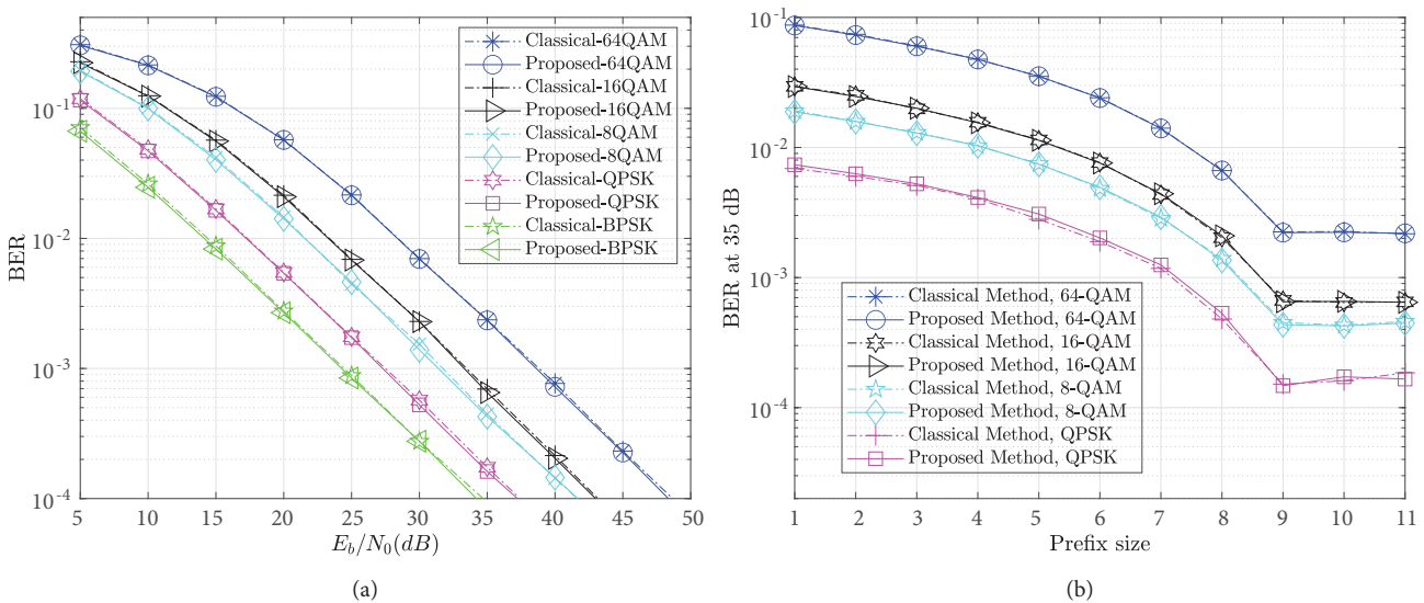
Figure 3. BER performances of the proposed scheme (with Algorithm-2) and conventional OFDM (a) for N = N_\alpha = 128 (b) for different prefix sizes N_{CP} at SNR= 35 dB.
