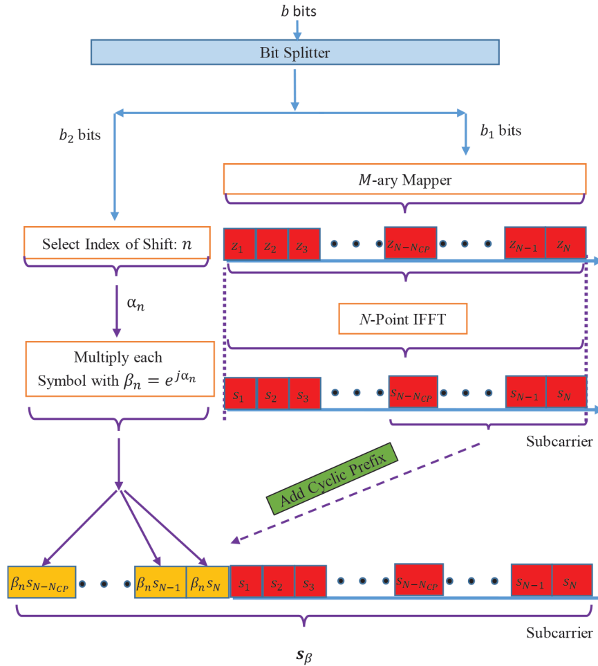
Figure 1. Frame structure of the proposed method.
