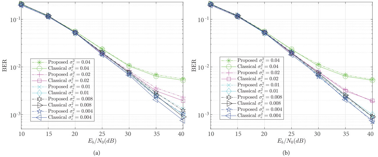
Figure 4. BER performances of the proposed scheme and conventional OFDM with 64-QAM and N = N_\alpha = 1024 under imperfect channel estimation error (a) for Algorithm-2 (b) for Algorithm-1.
