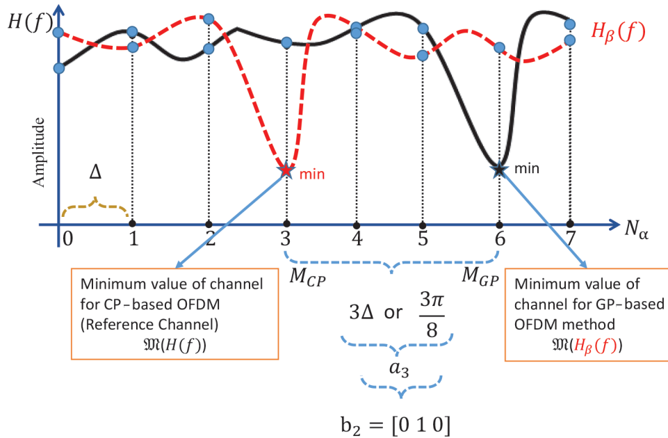
Figure 2. Frequency responses of CP- and GP-based channels with N_\alpha = 8 subcarriers.
