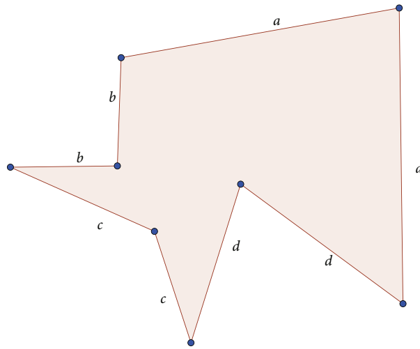
Figure 2. A flat sphere from a planer polygon.
