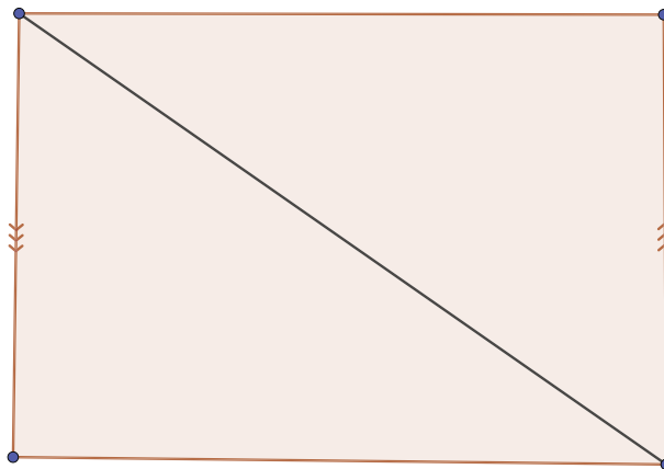
Figure 6. An ideal triangulation of the Möbius band with one labeled point.
