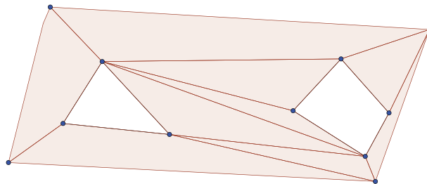
Figure 4. A singular flat surface which is homeomorphic to S^2[3] .
