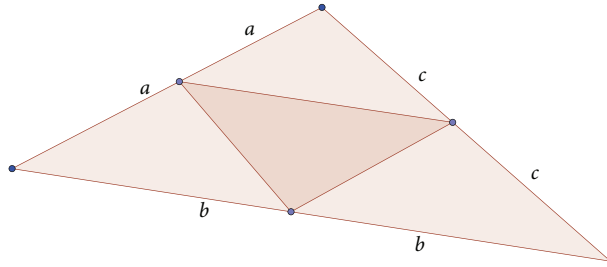
Figure 1. A triangulation of the flat sphere with four singular points.
