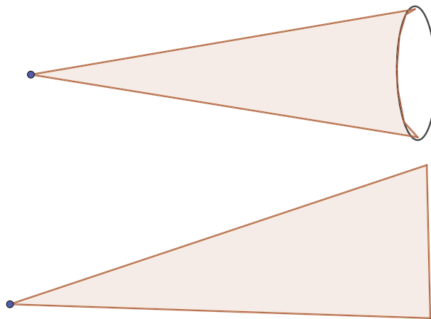
Figure 3. A cone and a cut of a cone.
