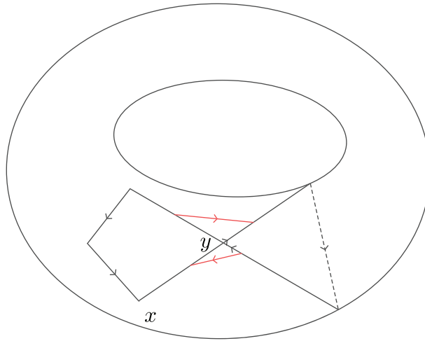
Figure 5. The polygonal loop \alpha is described in a torus. Consider the quadrilateral formed by red line segments. If we modify \alpha by replacing its diagonals by red segments, then we get a path whose length is strictly less than the length of \alpha .
