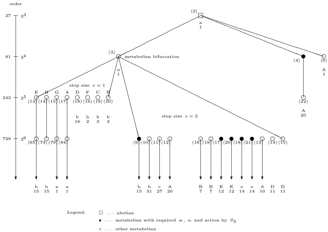
Figure 3. Finite 3-groups G with commutator quotient G/G' \simeq C_9 \times C_3 .
