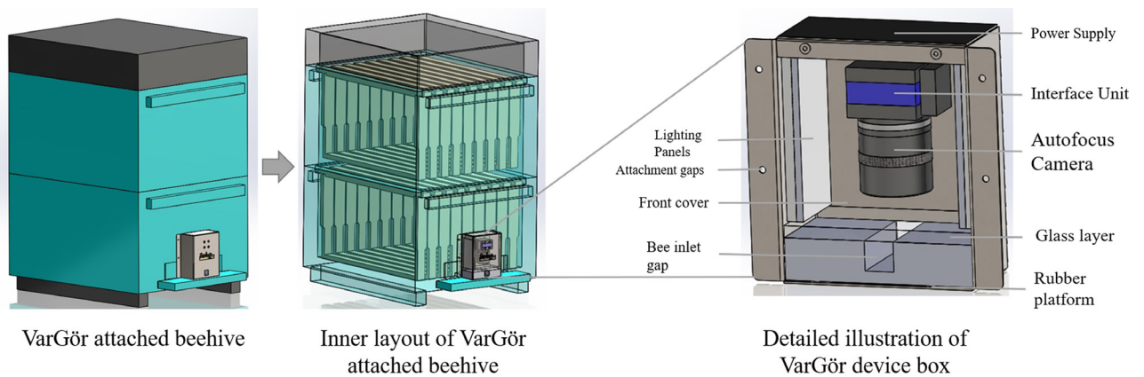
Figure 1. Interior design illustration of the Var-Gor device box.
