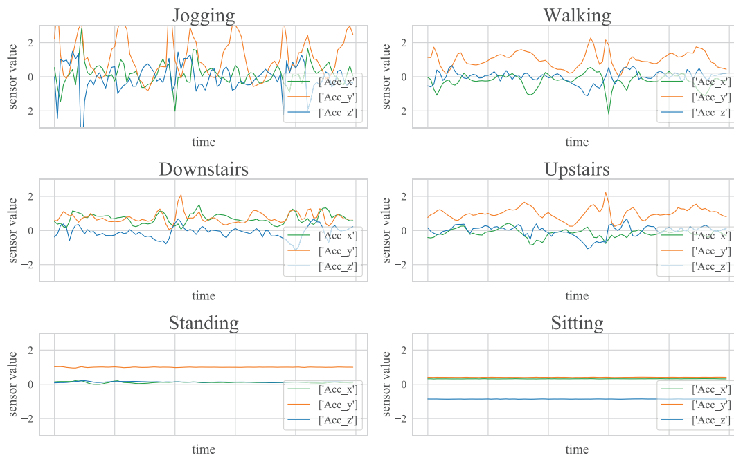
Figure 2. Sample accelerometer sensor signals in the x , y , z -axis over time for each activity.
