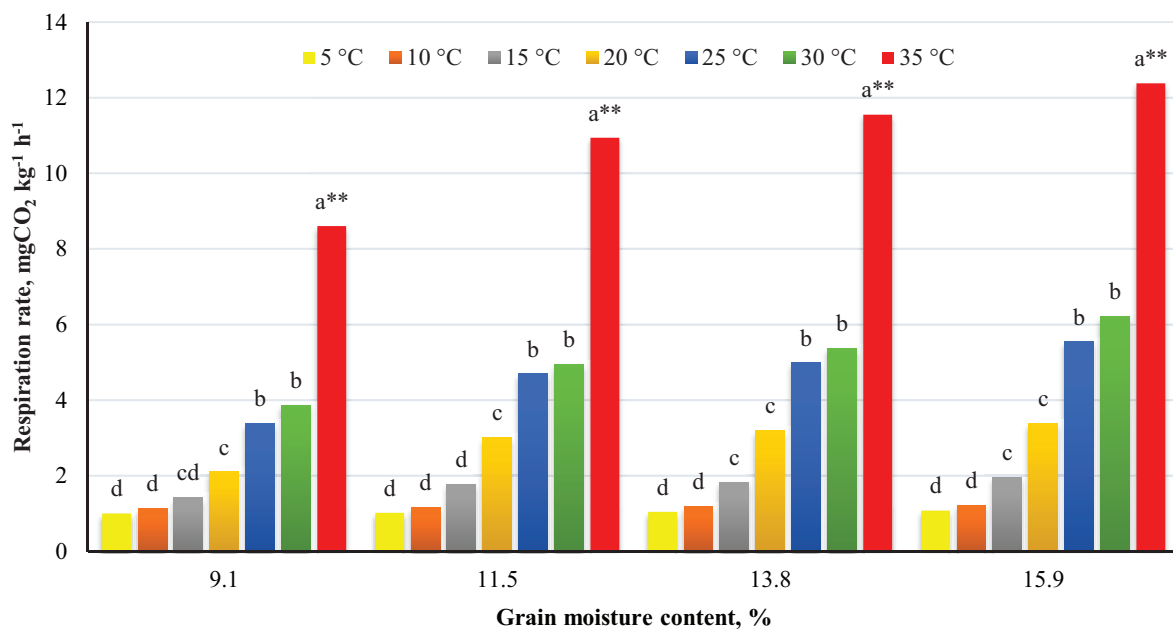
Figure 6. Respiration rates after 24 h depending on different temperature and grain moisture content (means were separated by using Tukey HSD multiple range test).
