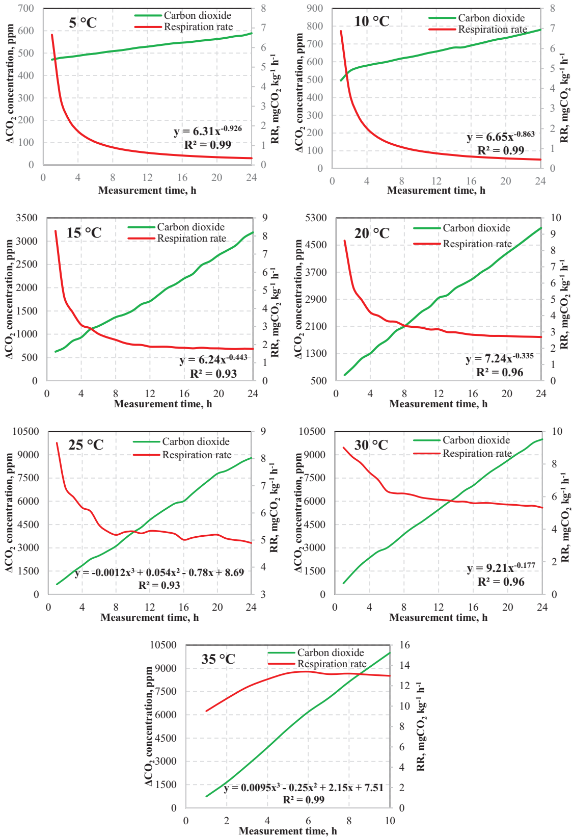
Figure 5. \text{CO}_2 concentrations and respiration rates as affected by 15.9% moisture content and temperature.
