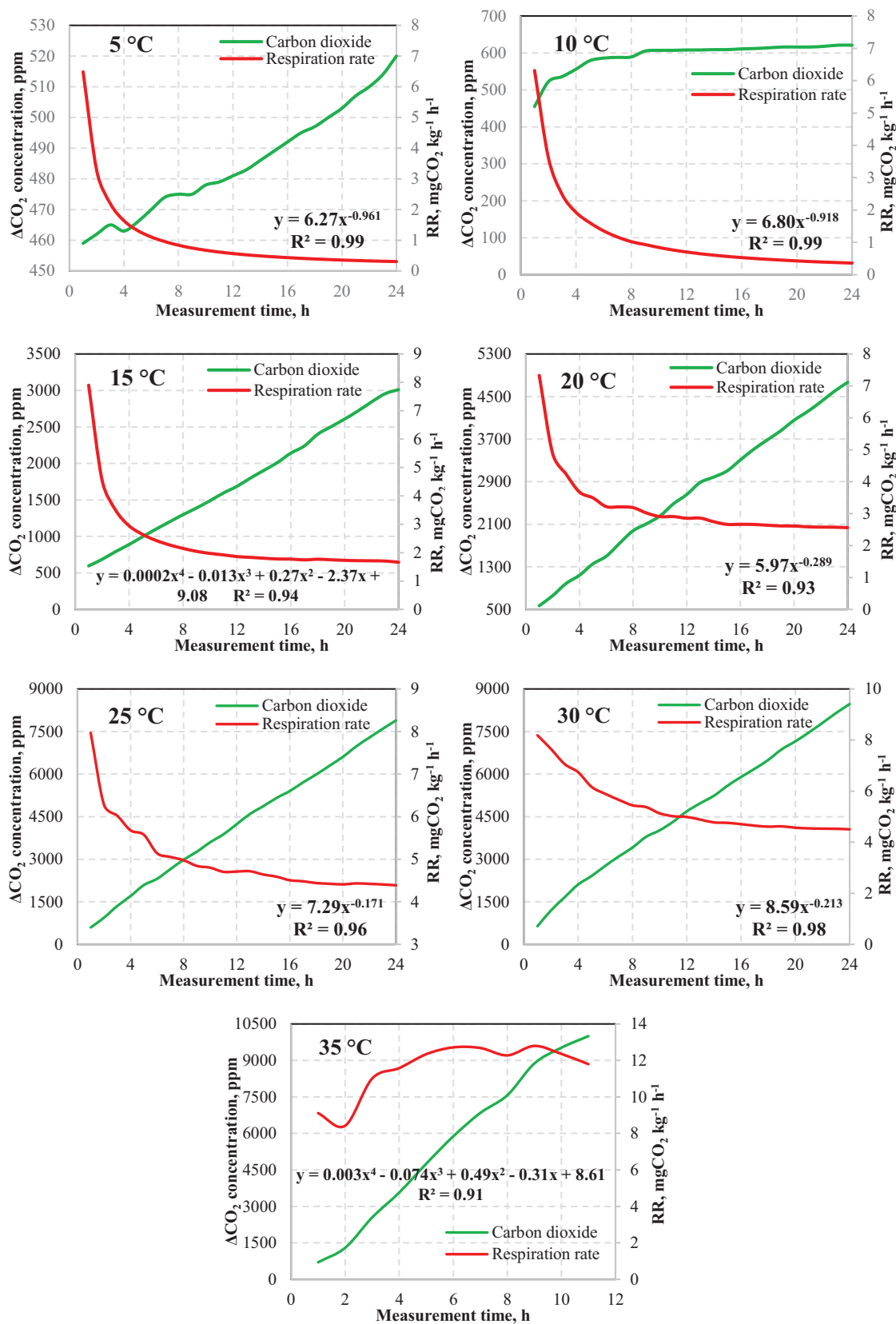
Figure 4. \text{CO}_2 concentrations and respiration rates as affected by 13.8% moisture content and temperature.
