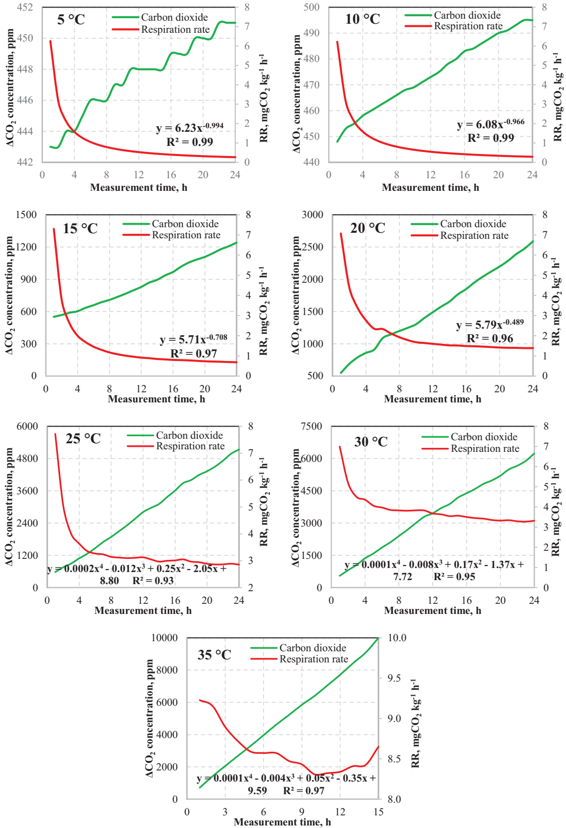
Figure 2. \text{CO}_2 concentrations and respiration rates as affected by 9.1% moisture content and temperature.
