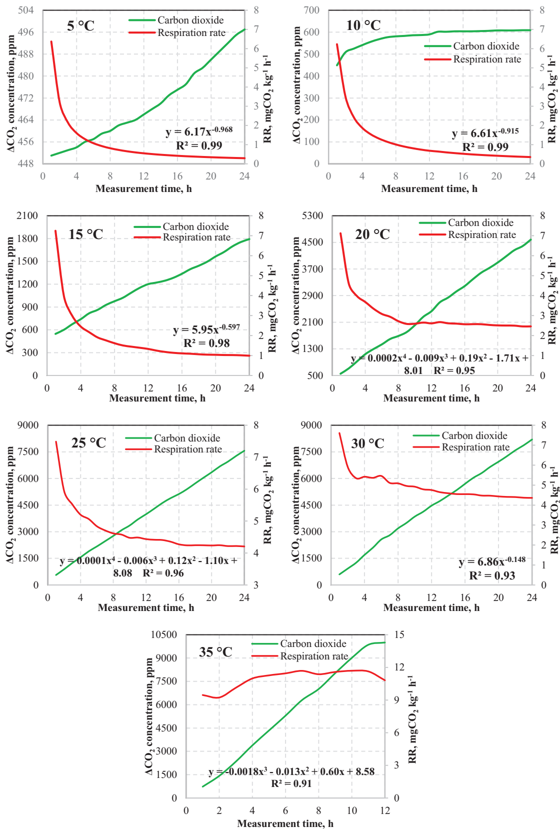
Figure 3. CO 2 concentrations and respiration rates as affected by 11.5% moisture content and temperature.
