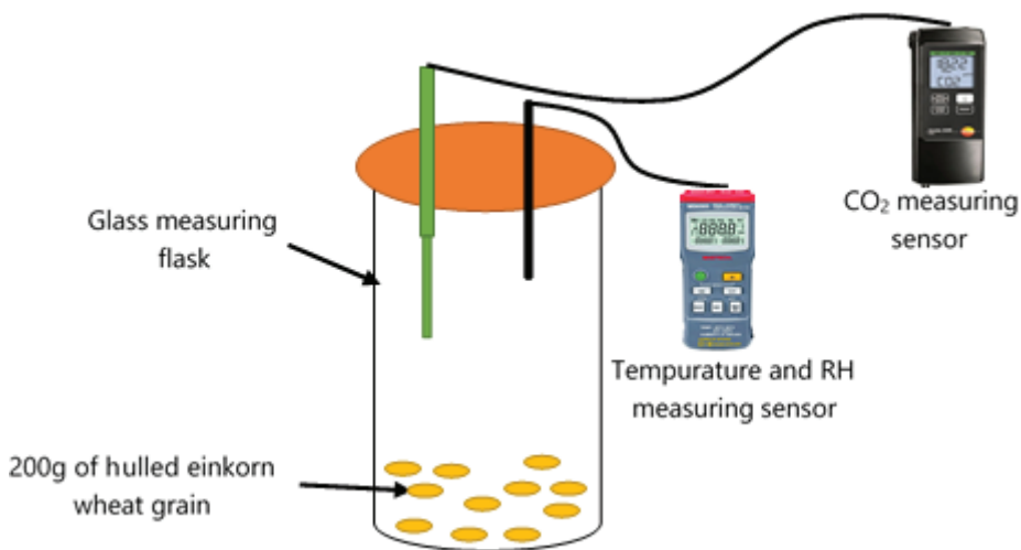
Figure 1. Experimental setup.
