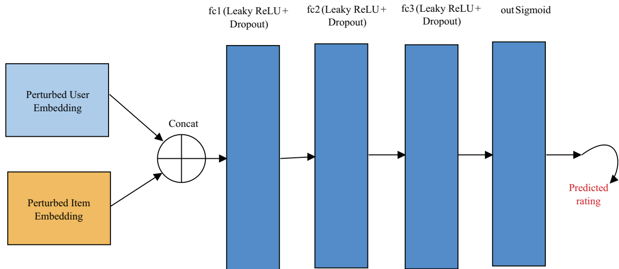
Figure 2. Proposed private hybrid recommendation system.
