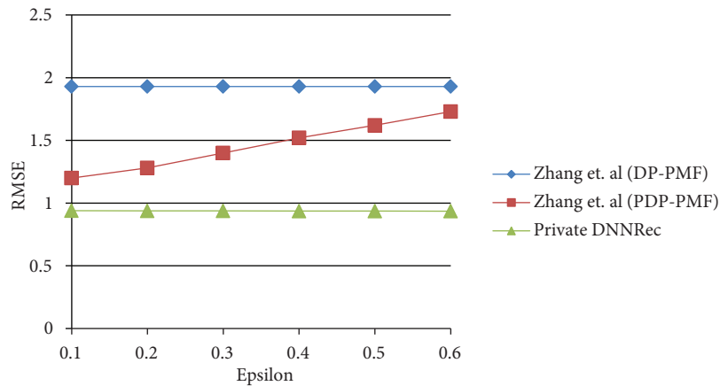
Figure 6. Comparison to other differential privacy based algorithm.
