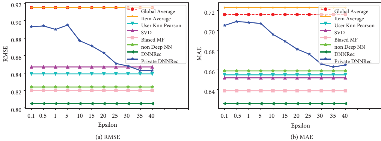
Figure 4. Accuracy of Film Trust.
