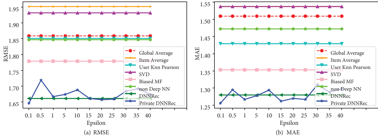
Figure 5. Accuracy of Book-Crossing.
