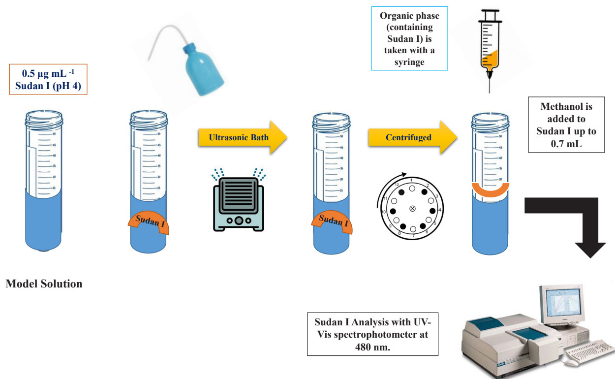
Figure 1. Schematic summary of the method developed.
