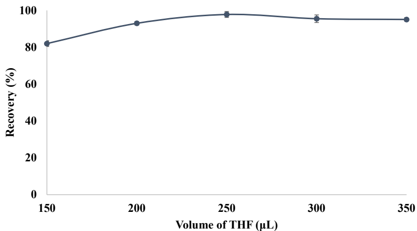
Figure 4. The effects of THF volume on the recovery value of the method (N = 3).
