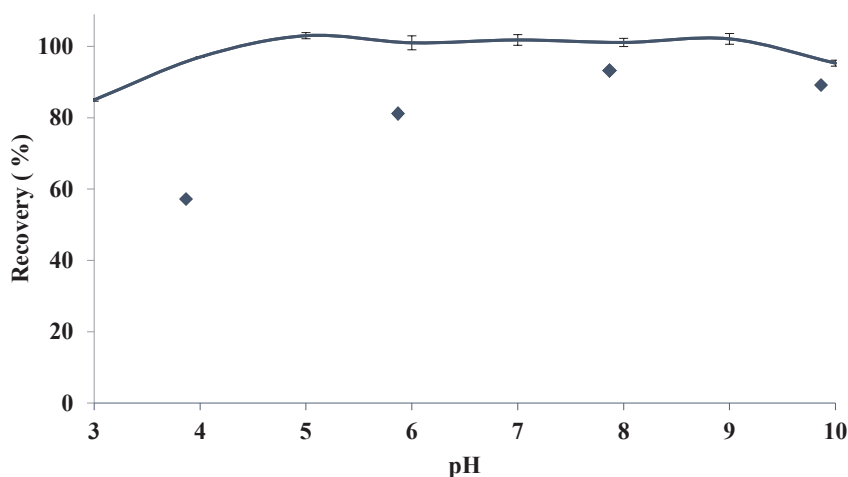
Figure 2. Influence of pH value of extraction recovery (N = 3).
