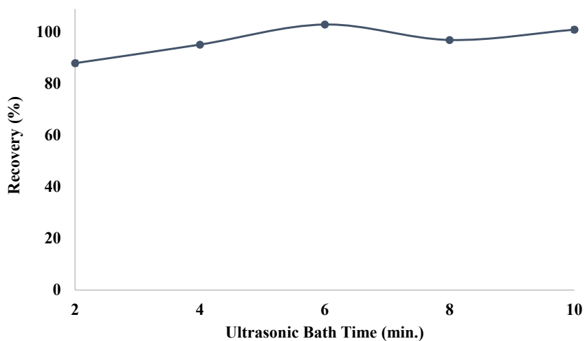
Figure 5. Influences of ultrasonic bath time on the recovery value of the method (N = 3).
