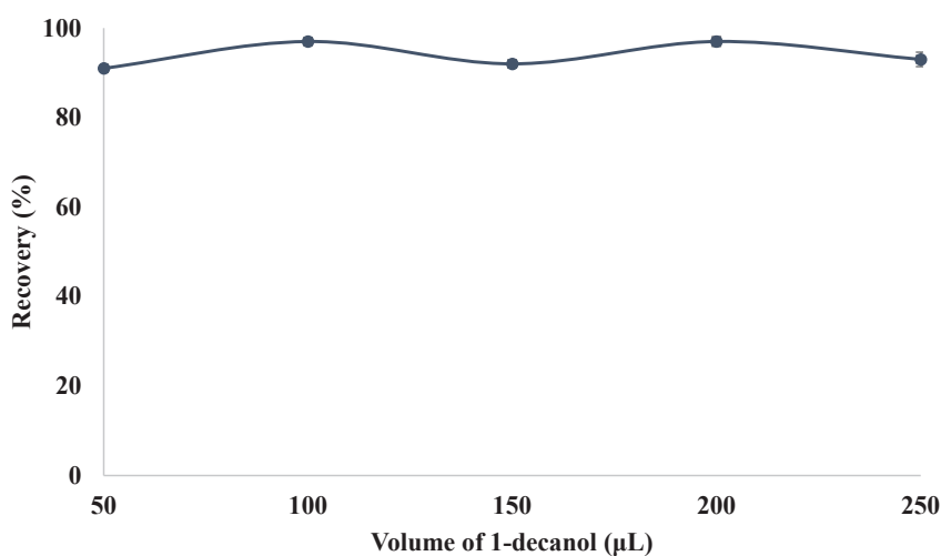
Figure 3. The effect of 1-decanol on the recovery yield efficiency of the developed method (N = 3).
