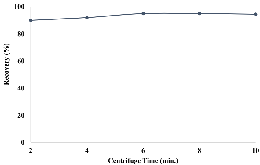
Figure 6. Effects of centrifuge time on the recovery value of the method (N = 3).
