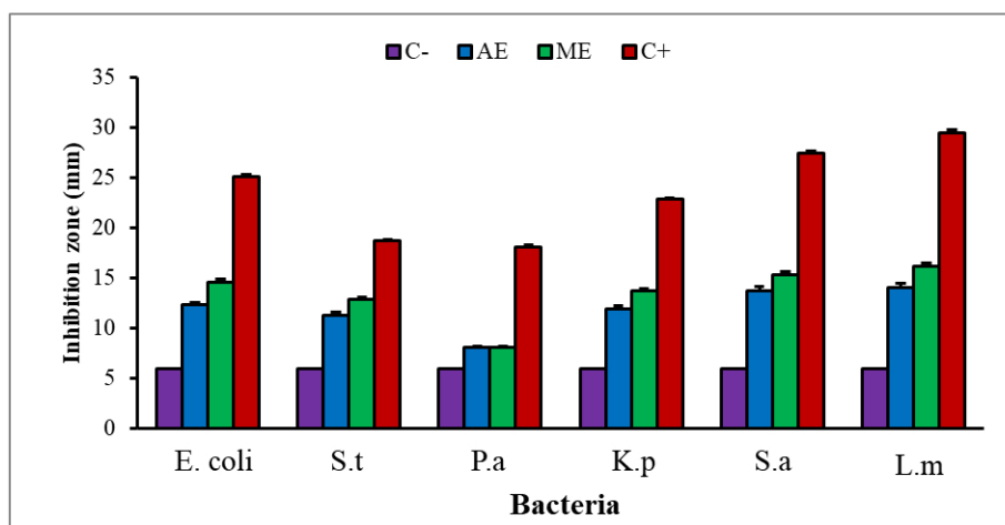
Figure 1. Inhibition zones (the vertical bars represent standard deviation of the means) created by aqueous and methanol extracts of E. guttatum against the studied bacteria. E. coli : Escherichia coli ATCC 25922; K.p : Klebsiella pneumonia ATCC 43816; P.a : Pseudomonas aeruginosa ATCC 27853; S.t : Salmonella typhimurium ATCC 14028; L.m : Listeria monocytogenes ATCC 13932; S.a : Staphylococcus aureus ATCC 25923; C-: negative control (methanol); C+: positive control (Gentamicin, 30 µg).
