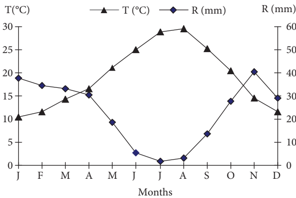
Figure 2. Climate diagram of the Lower Cheliff.
