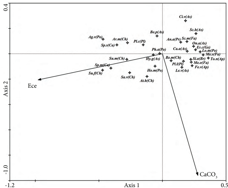
Figure 5. Redundancy analysis of 29 species and 2 explanatory variables at 133 relevés in the plain of Lower Cheliff. Both axes of the ordination plot explain 8.9% of the species variance and 100% of the species-environment relation.
