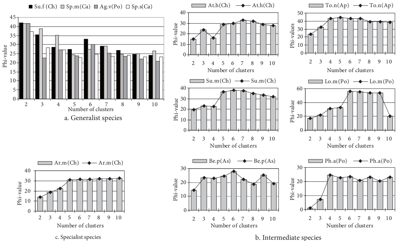
Figure 4. Evolution of the phi coefficient for 10 subdivisions. For species abbreviations, see Table 1.
