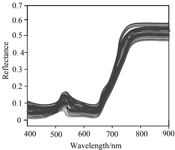
Figure 4. The spectral curve of rapeseed sample for chlorophyll b detection. (a) Modeling set. (b) Prediction set.
