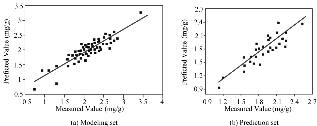
Figure 7. Scatter plot of full-spectrum PLS model for prediction of total chlorophyll.
