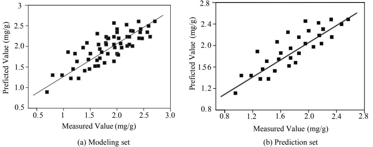
Figure 3. Scatter plot of full-spectrum PLS model for prediction of chlorophyll a.
