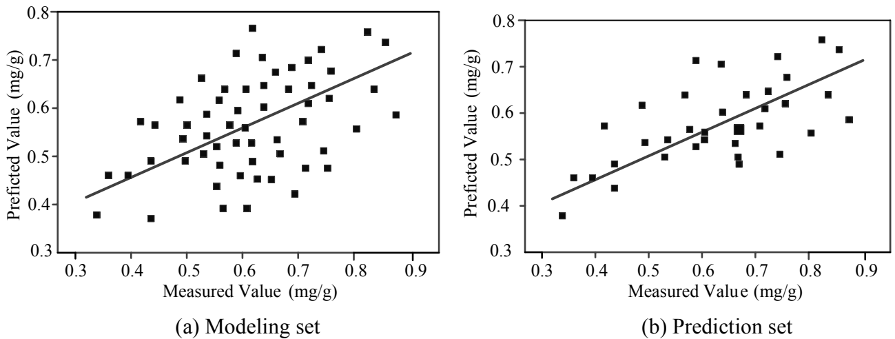
Figure 5. Scatter plot of full-spectrum PLS model for prediction of chlorophyll a.
