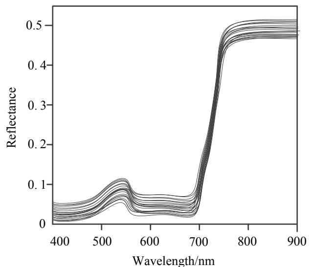
Figure 2. The spectral curve of rapeseed sample for chlorophyll detection. (a) Modeling set. (b) Prediction set.
