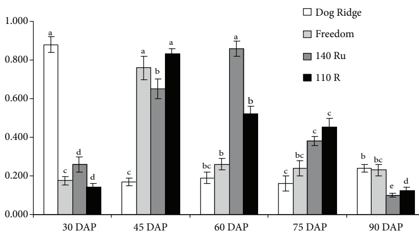
Figure. PPO activity ( \text{EU mL}^{-1} \text{min}^{-1} ) in grape rootstocks during rooting.
