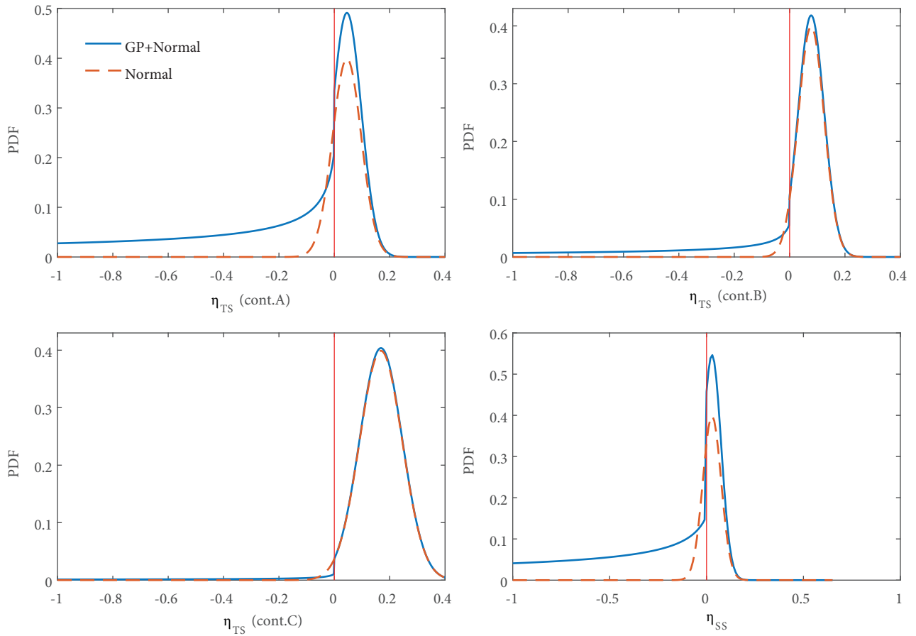
Figure 4. Probability density functions (PDFs) for dynamic performances.
