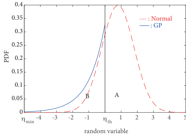
Figure 2. Combination of generalized Pareto and normal distributions.
