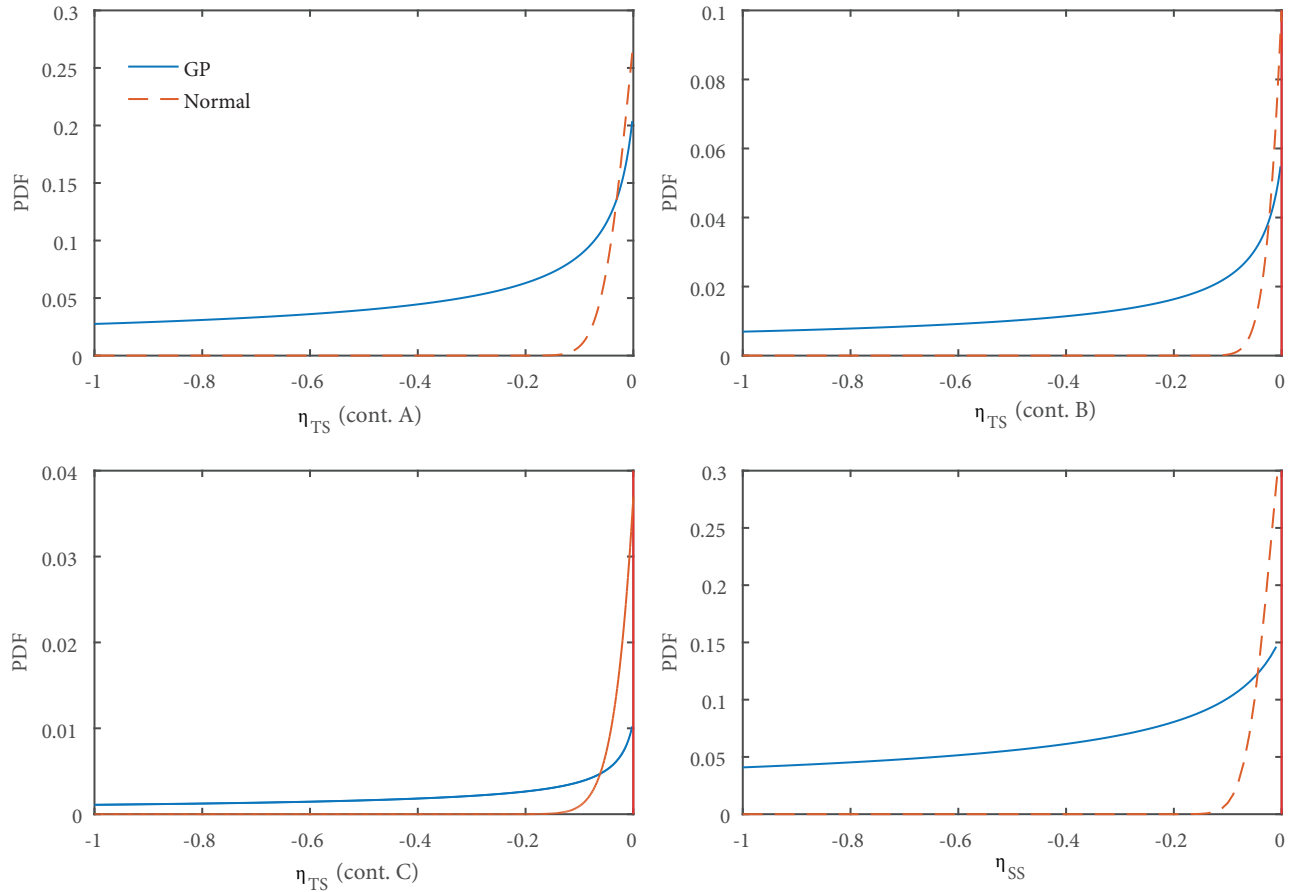
Figure 5. Probability density functions (PDFs) over the tailed region (ES).
