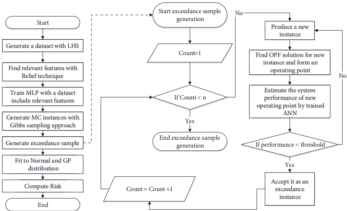
Figure 1. Flowchart of the proposed method including exceedance sample generation.
