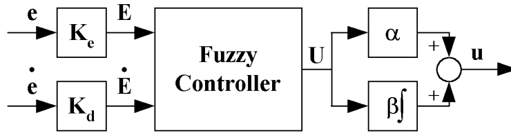
Figure 1. Two-input FPID controller structure with one rule-base.
